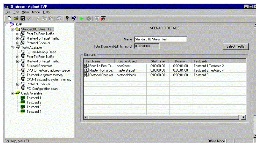
Figure 3. Test scenario setup window
