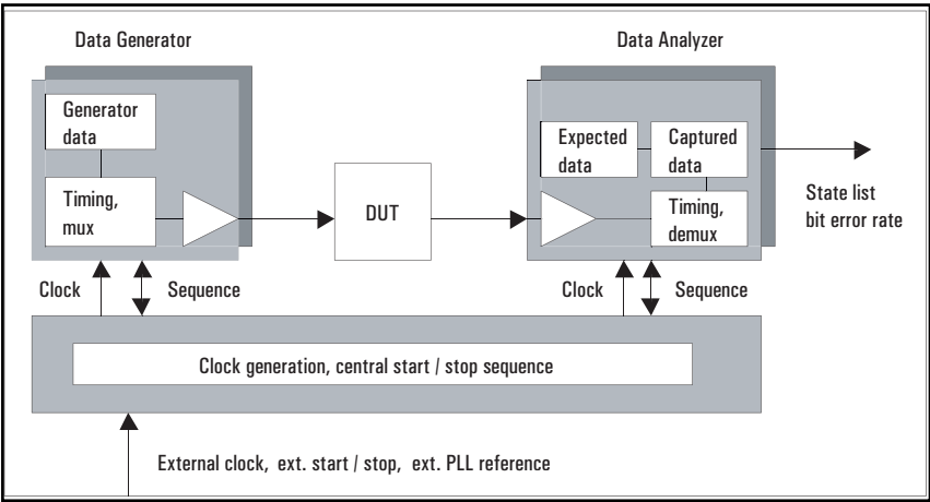
Figure 2: Block Diagram of 81200 functional layout
