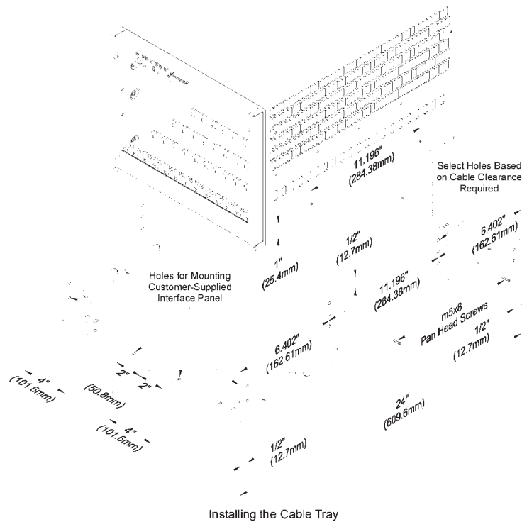
Installing the Cable Tray
