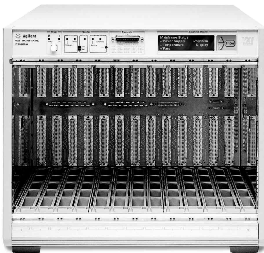
Agilent E8404A
