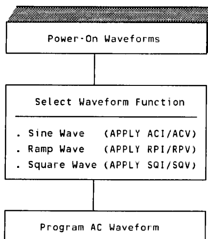
Figure 11-2. Power-On AC Waveforms - Selection Steps
