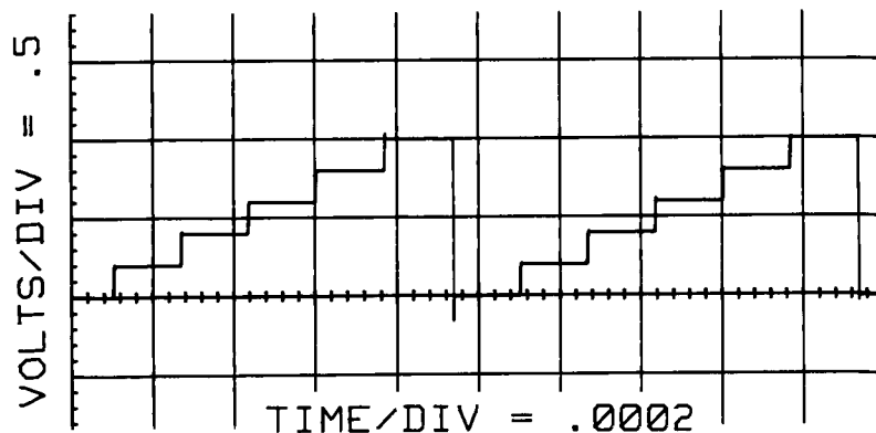
Figure 5-5. Example: Linear Steps
