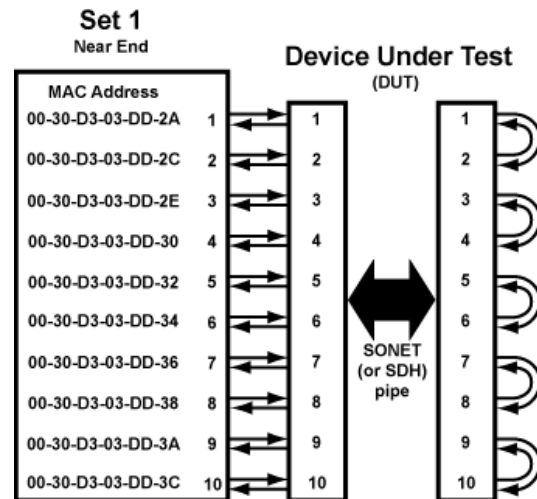
Port-to-Port Loopback
