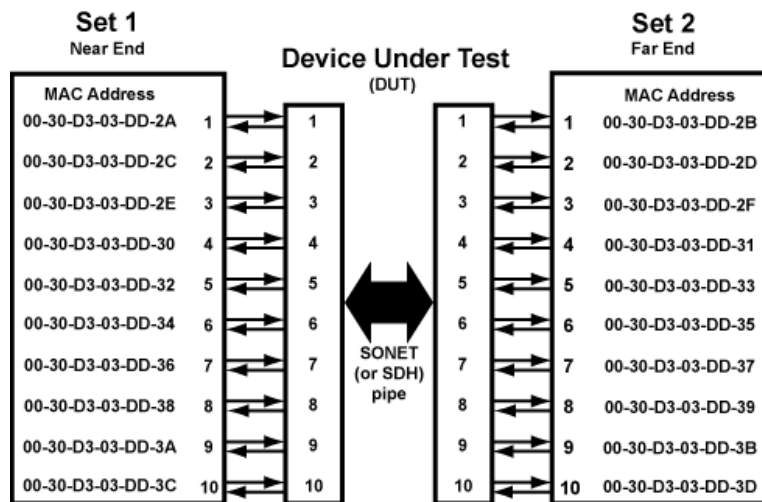
End-to-End Testing
