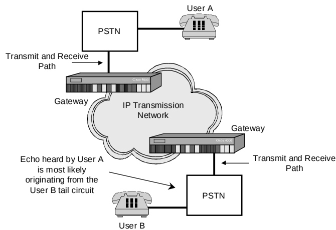
Figure 5: Echo originates from the far-end tail circuit.
