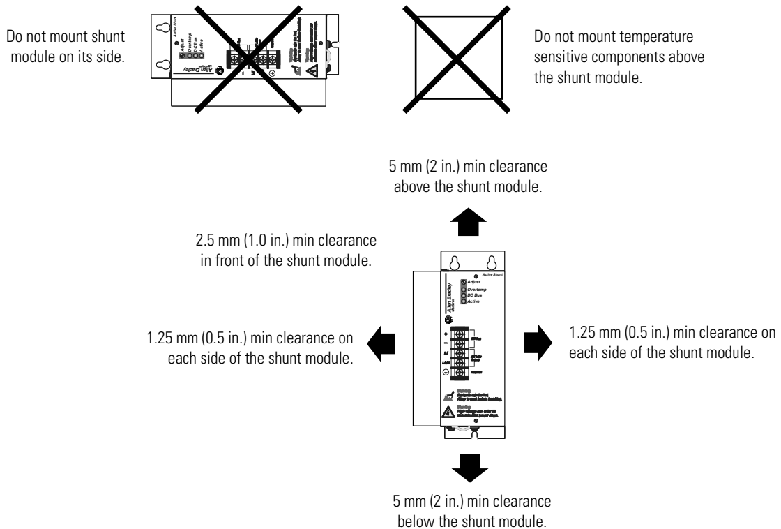
Figure 4 Shunt Module Spacing Requirements within an Enclosure
