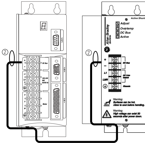
Figure 6 DC Bus Wiring Layout Using Ferrites with Shielded Cable
