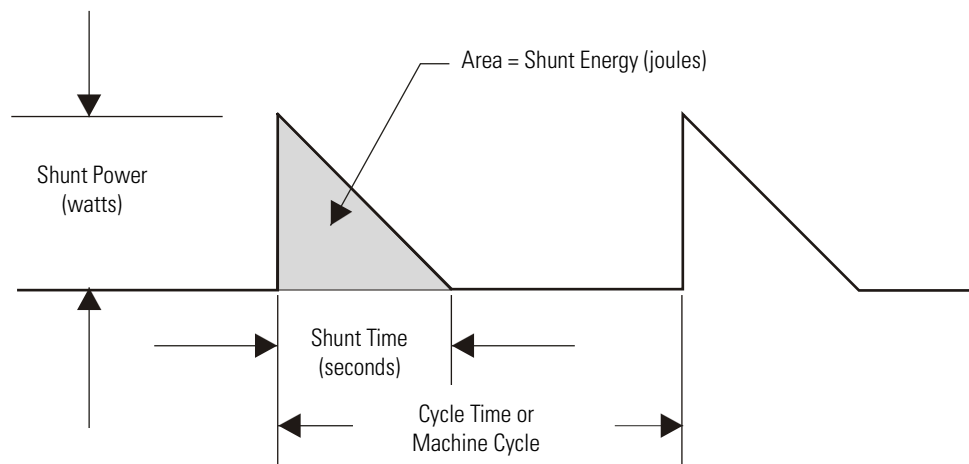
Figure 2 Shunt Regeneration Profile
