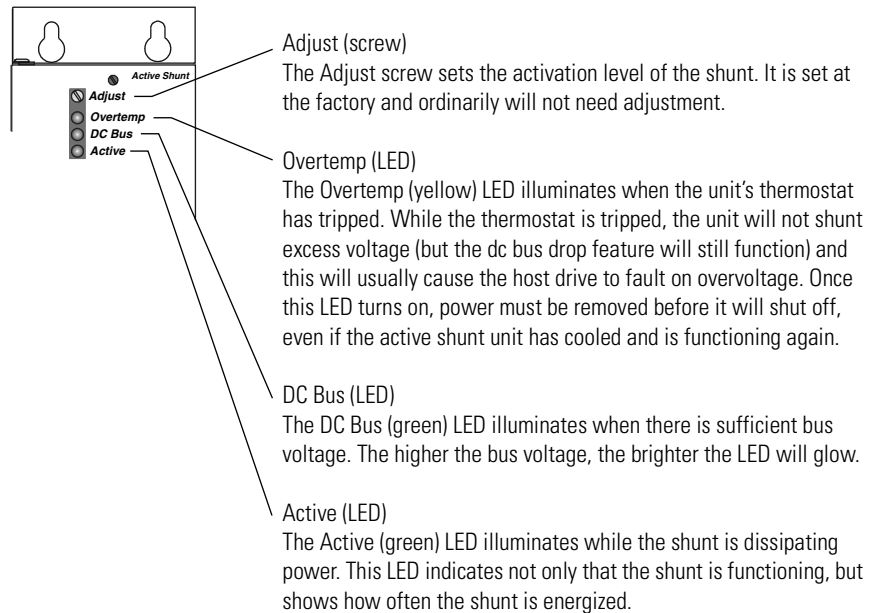
Figure 7 Shunt Module Adjustment Screw and LEDs
