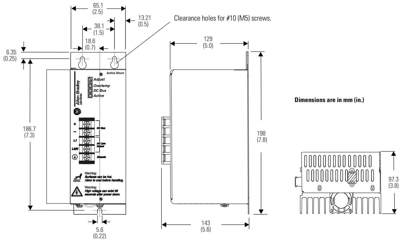
Figure 5 300 W Active Shunt Regulator Mounting Dimensions
