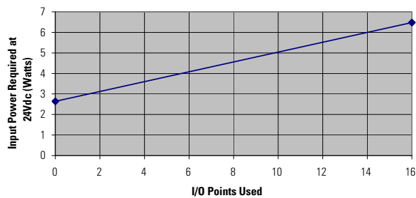
1761-L16BWB Typical Power Requirements
