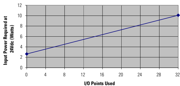
1761-L32BWB Typical Power Requirements
