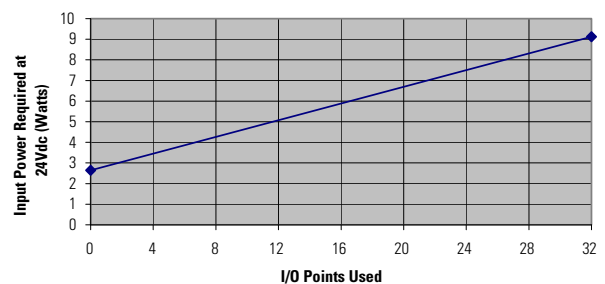
1761-L32BBB Typical Power Requirements
