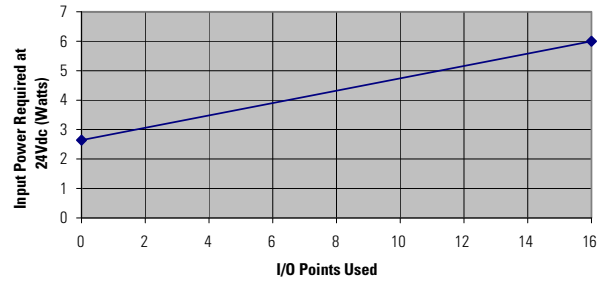
1761-L10BXB, -L16BBB, Typical Power Requirements
