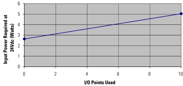
1761-L10BWB Typical Power Requirements
