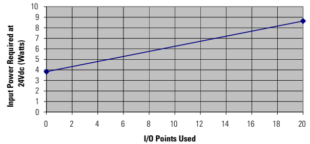
1761-L20BWB-5A Typical Power Requirements
