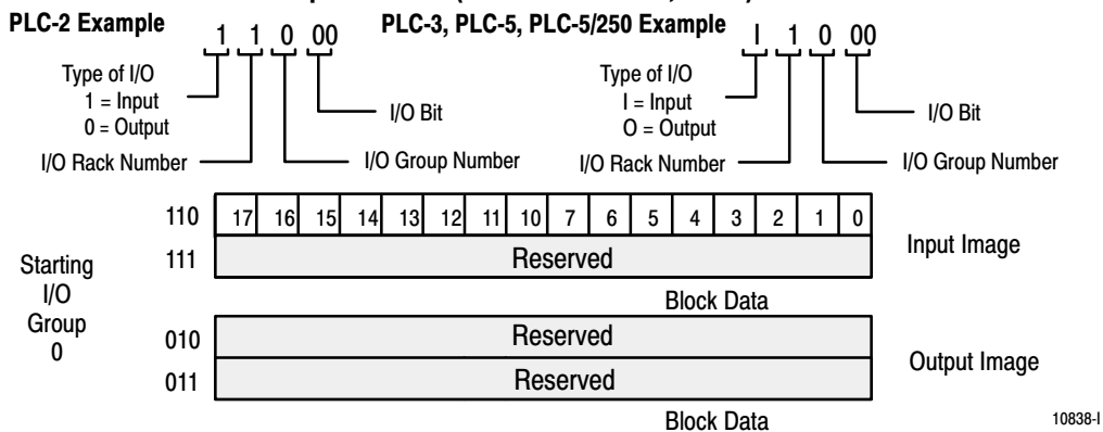
Figure 4.4 Input/Output Image Table Usage Example for One Starting I/O Group with 16 Input Modules (cat. no. 1791-16A0, -16B0)
