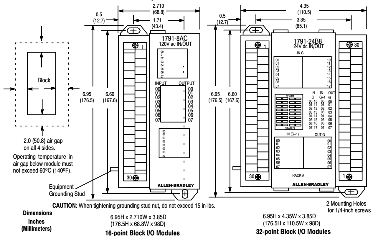
Figure 3.1 Mounting Dimensions for the Block I/O Modules
