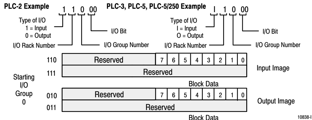
Figure 4.5 Input/Output Image Table Usage Example for One Starting I/O Group for 8 Input/8 Output Modules (cat. no. 1791-8AC, -8BC, -8AR, -8BR)
