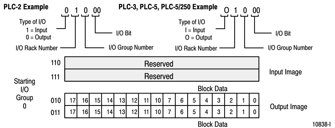
Figure 4.7 Input/Output Image Table Usage Example for One Starting I/O Group for 32 Output Modules (cat. no. 1791-0A32, -0B32)
