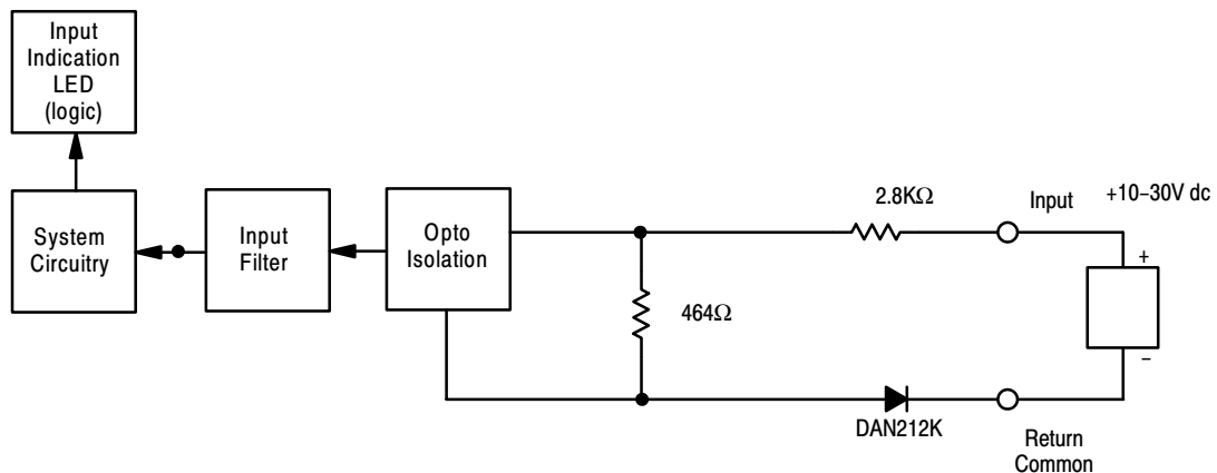
Figure 2.4 Simplified Schematic of Sinking dc Input Circuit
