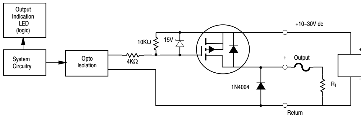
Figure 2.9 Simplified Schematic of dc Output Circuit
