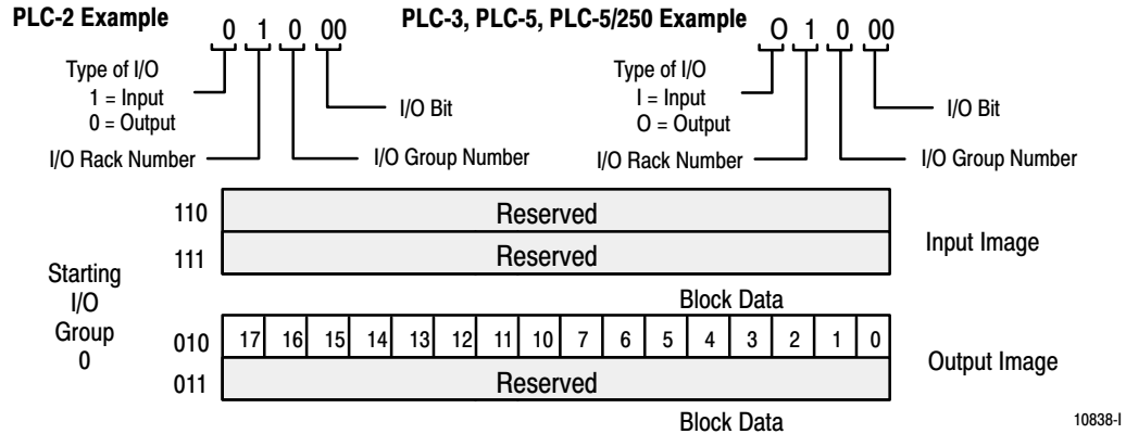
Figure 4.3 Input/Output Image Table Usage Example for One Starting I/O Group for 16 Output Modules (cat. no. 1791-0A16, -0B16)
