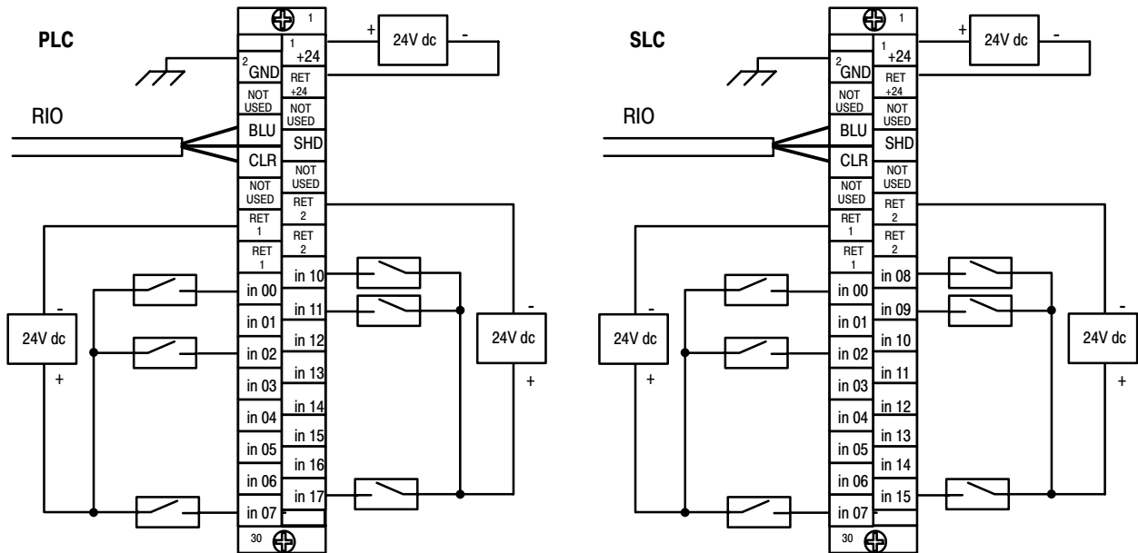
Figure 3.14 Input Wiring Connections for the 1791-16B0 Series B
