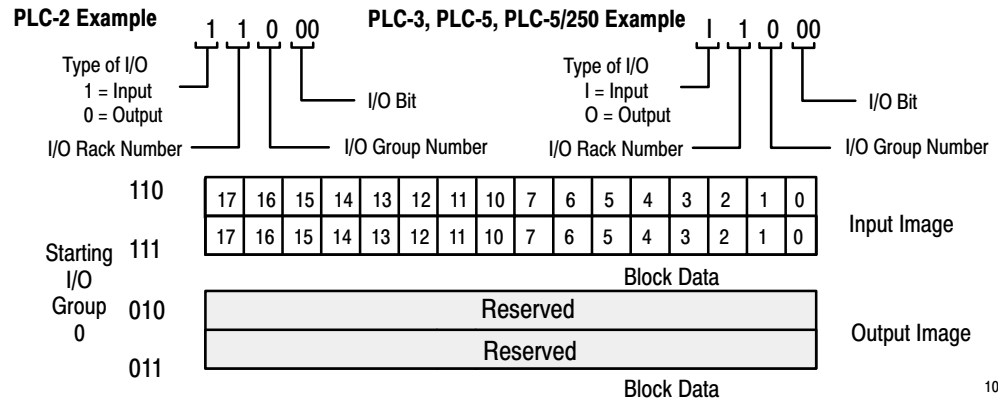
Figure 4.8 Input/Output Image Table Usage Example for One Starting I/O Group with 32 Input Modules (cat. no. 1791-32A0, -32B0)
