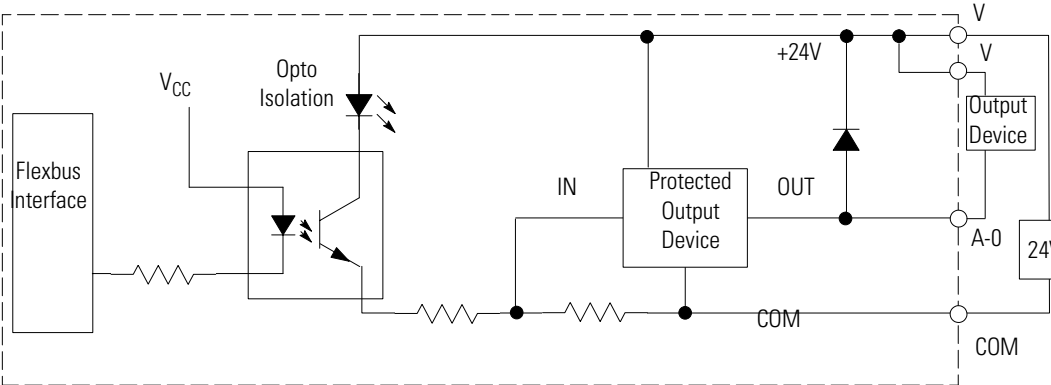
Typical Simplified Schematic for Output 0
