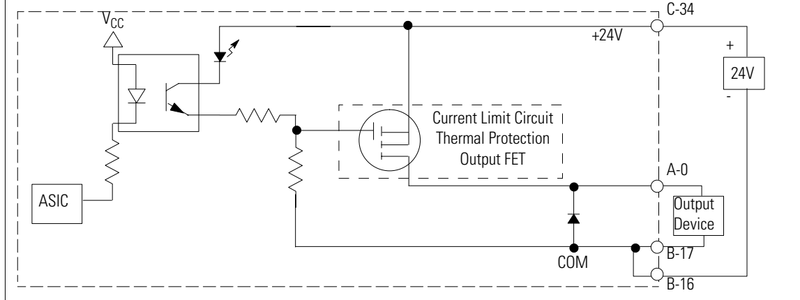
Typical Simplified Schematic for Output 0 TB3, TB3S, or TB2 shown
