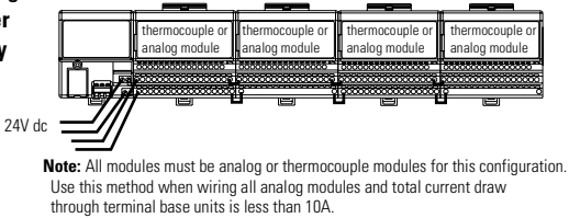
Wiring when total current draw is less than 10A
