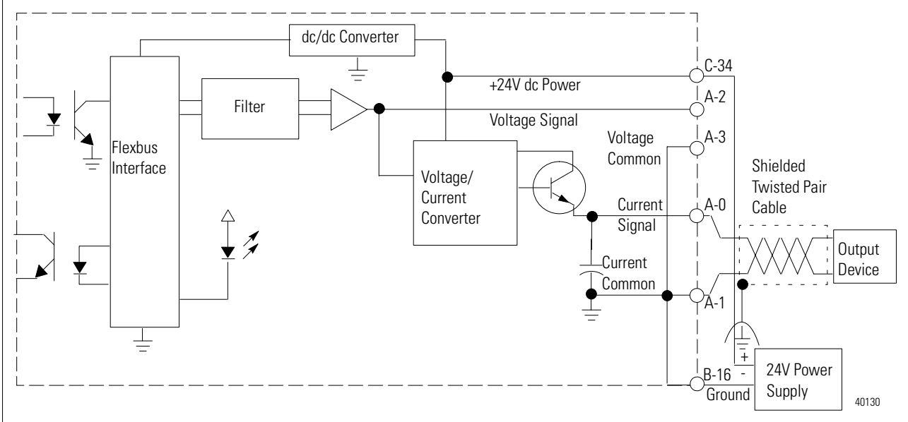
Simplified Schematic of Current Output 0 TB3, TB3S, TB2, TB3T, or TB3TS shown
