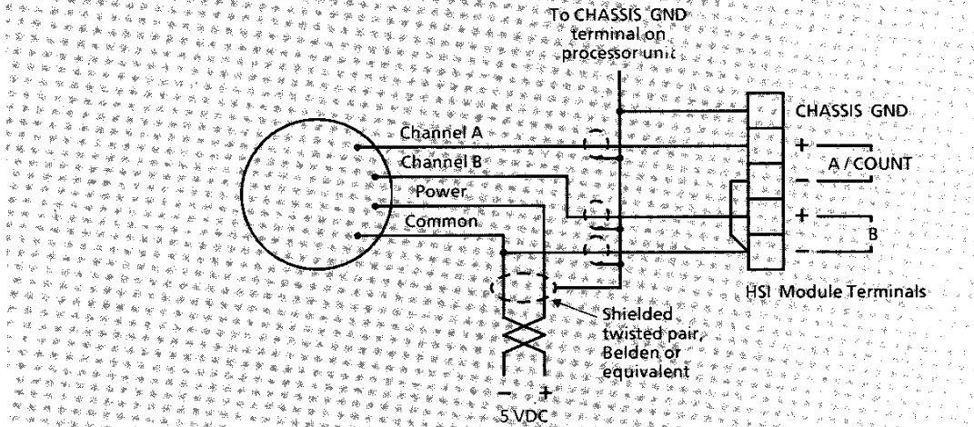
Single-ended wiring connections for a Bulletin 845N encoder
