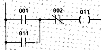
A typical hold-in rung
