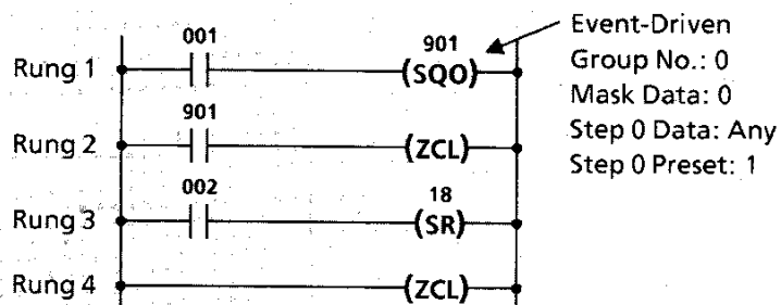
Event-driven shift right register
