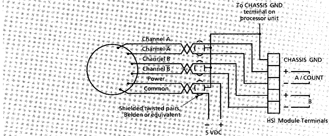
Differential wiring connections for a Bulletin 845N encoder
