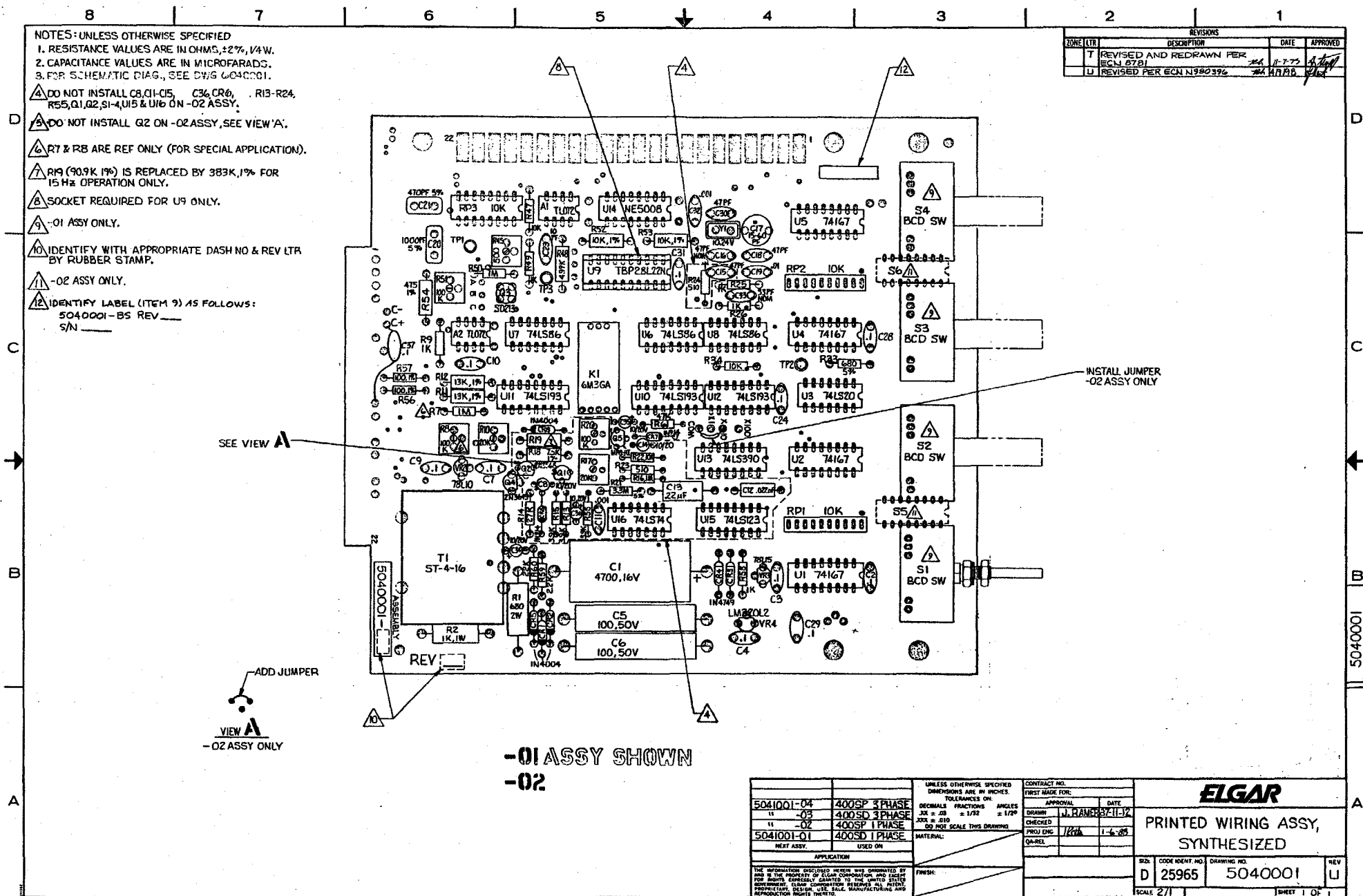
Figure 5-2. Model 400SD/SP Main Board Assembly Drawing
