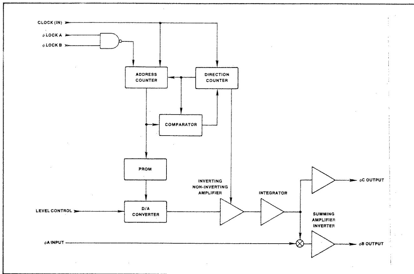
Figure 3-2. Block Diagram, Multi-Phase Generator Board.
