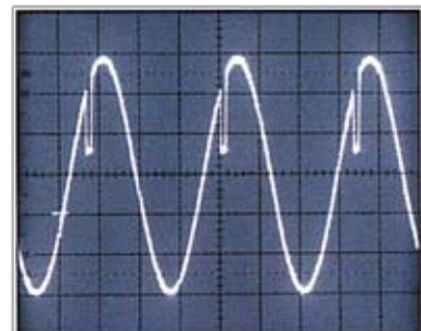
Sine wave with a dropout from 45°-60°.
