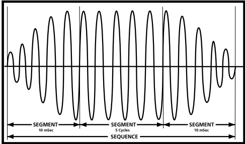
Sequences can be constructed with segments defined by time or number of cycles.
