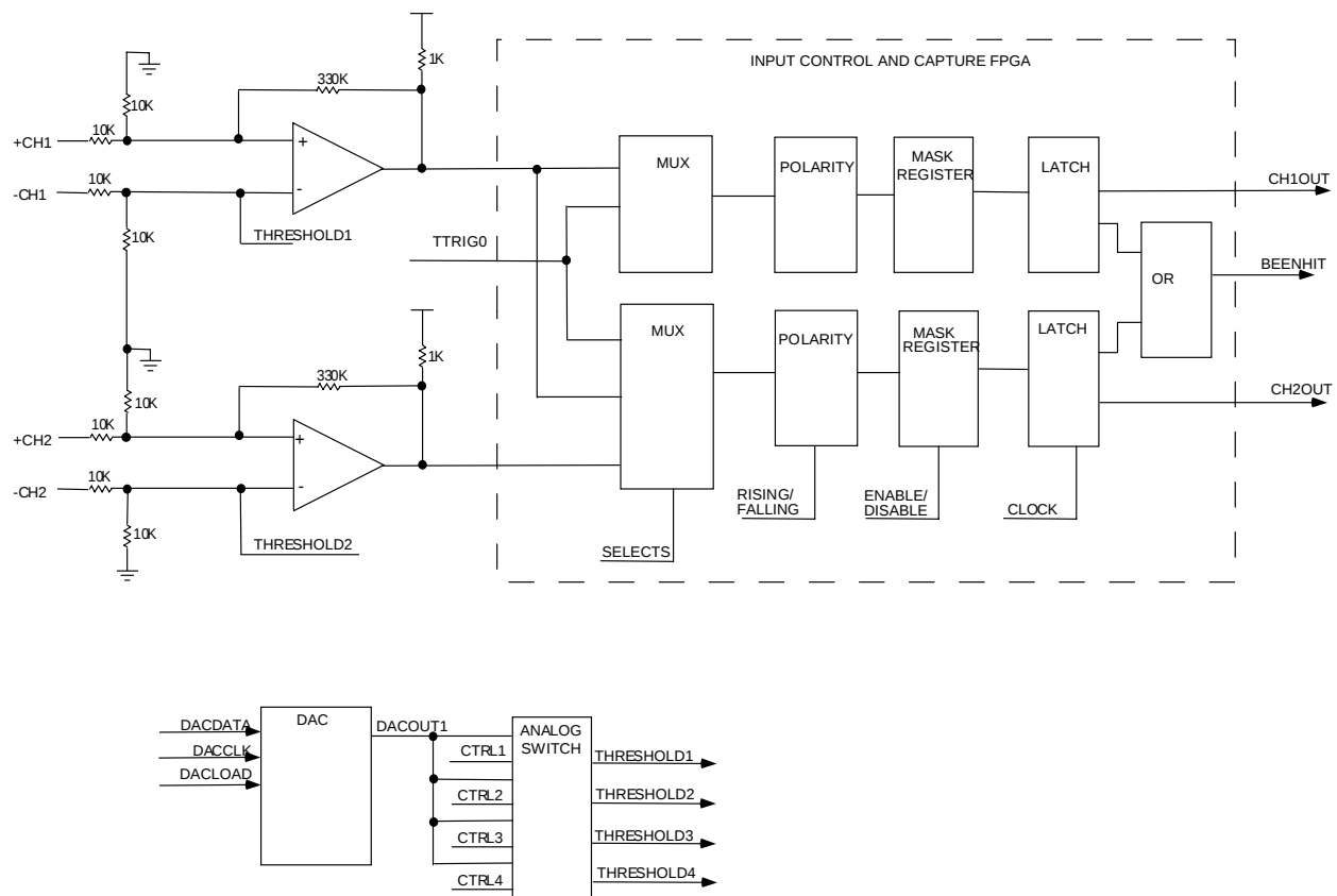
FIGURE 5-2 INPUT CONTROL AND CAPTURE FPGA BLOCK DIAGRAM
