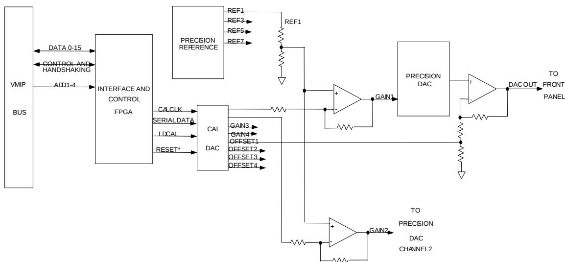
FIGURE 5-3: REFERENCE AND CALIBRATION FUNCTIONAL DIAGRAM
