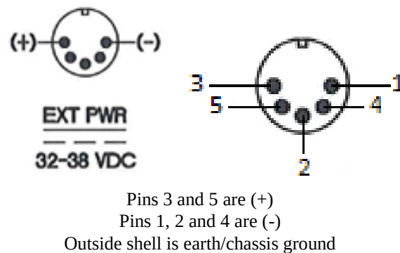
Figure 1: External Power Connector and Pin Numbers
