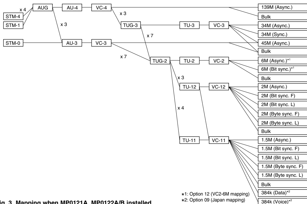
Fig. 3 Mapping when MP0121A, MP0122A/B installed
