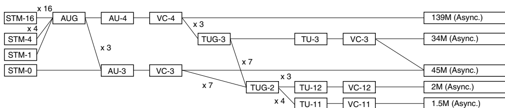
Fig. 4 Add/Drop mapping structure
