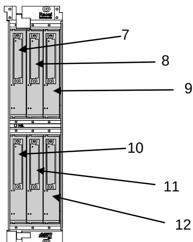
Front View – Module Addresses for 1260-100 Carrier
