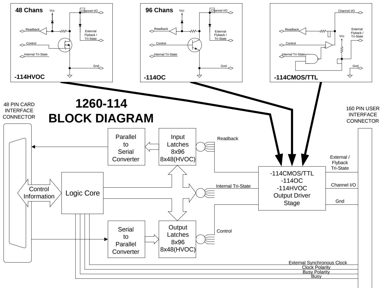
Figure 2-2, Block Diagram
