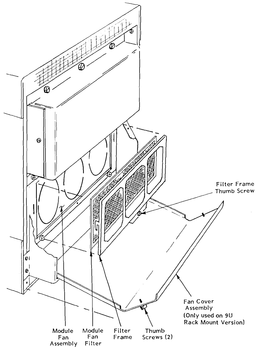
Figure 5-2 Cleaning The Module Fan Filter
