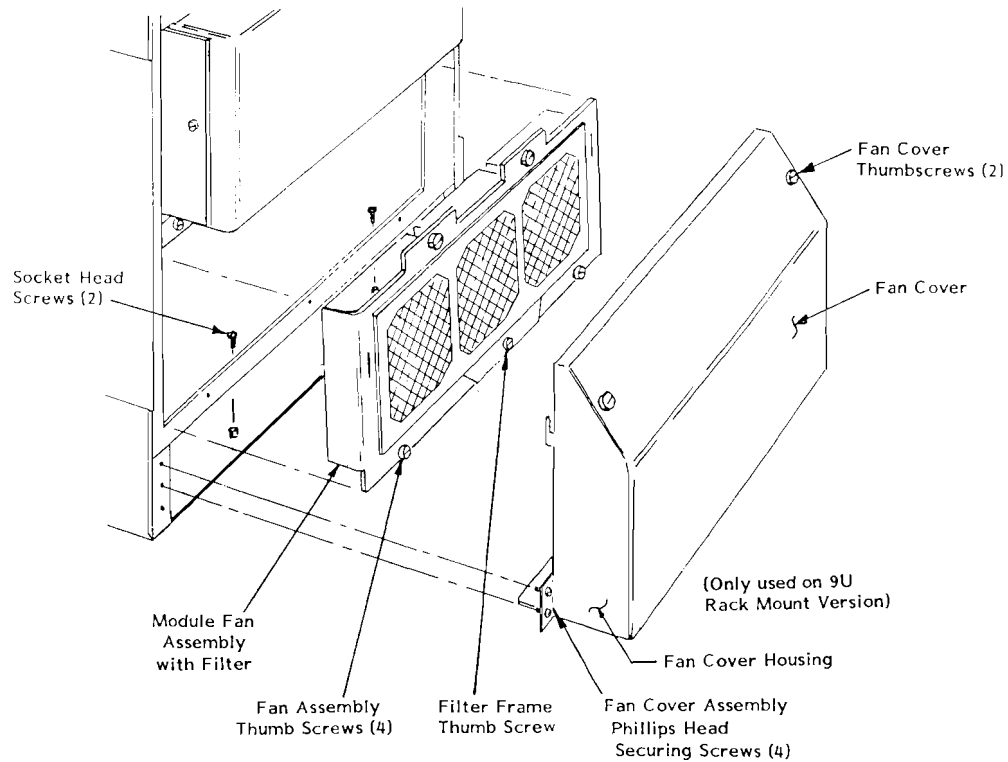
Figure 5-3 Module Fan Assembly Detail
