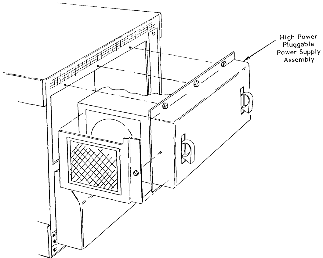
Figure 1-4 1261B/BL High Power Pluggable Power Supply
