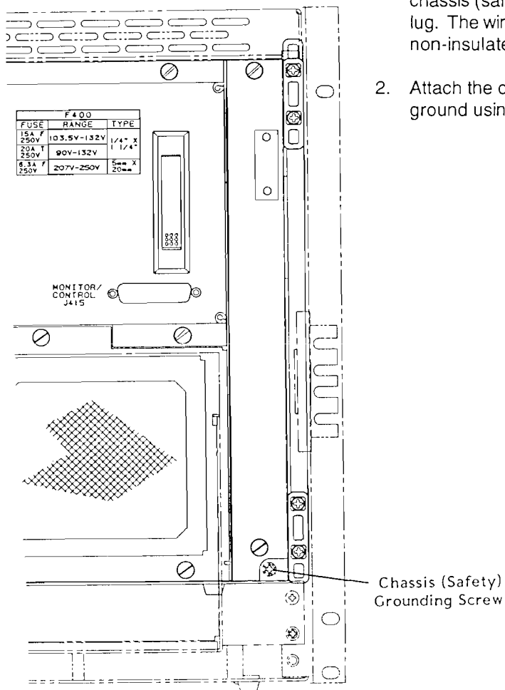
Figure 2-11 Connecting Safety Ground
