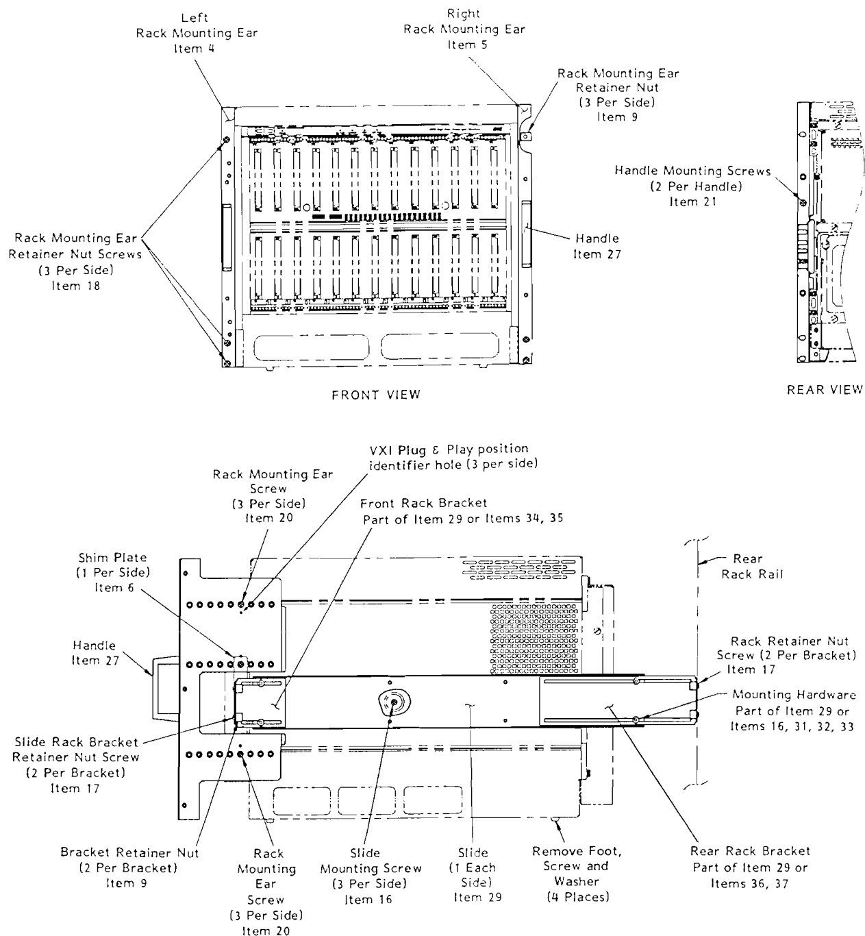
Figure 2-5 Preparing The Mainframe For Rack Mounting
