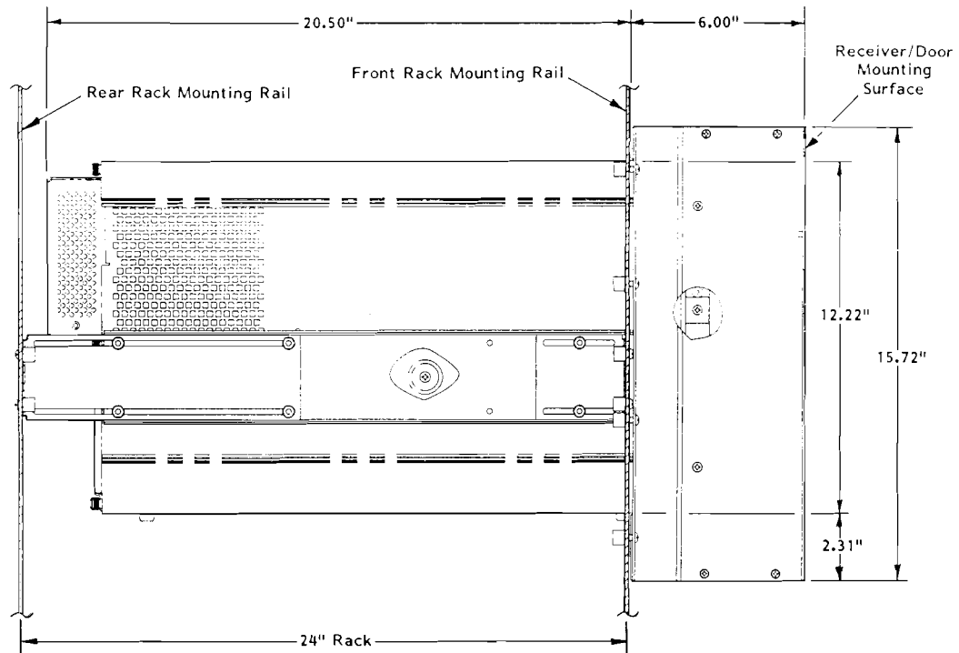
Figure A-5 Side View of 1261B/BL 7U Mainframe With Option 54-1 Installed
