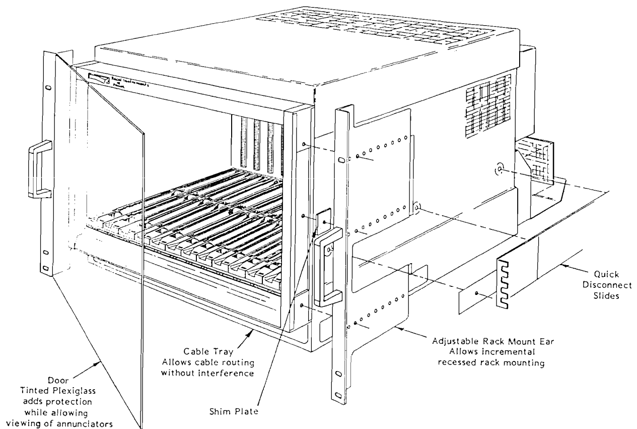
Figure 2-3 Rack Mount Options Major Components (9U Mainframe shown)
