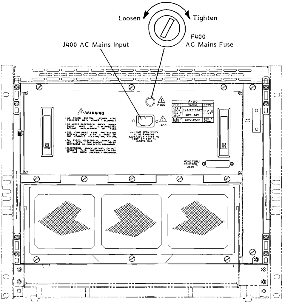
Figure 5-7 Removing and Replacing The AC Mains Fuse
