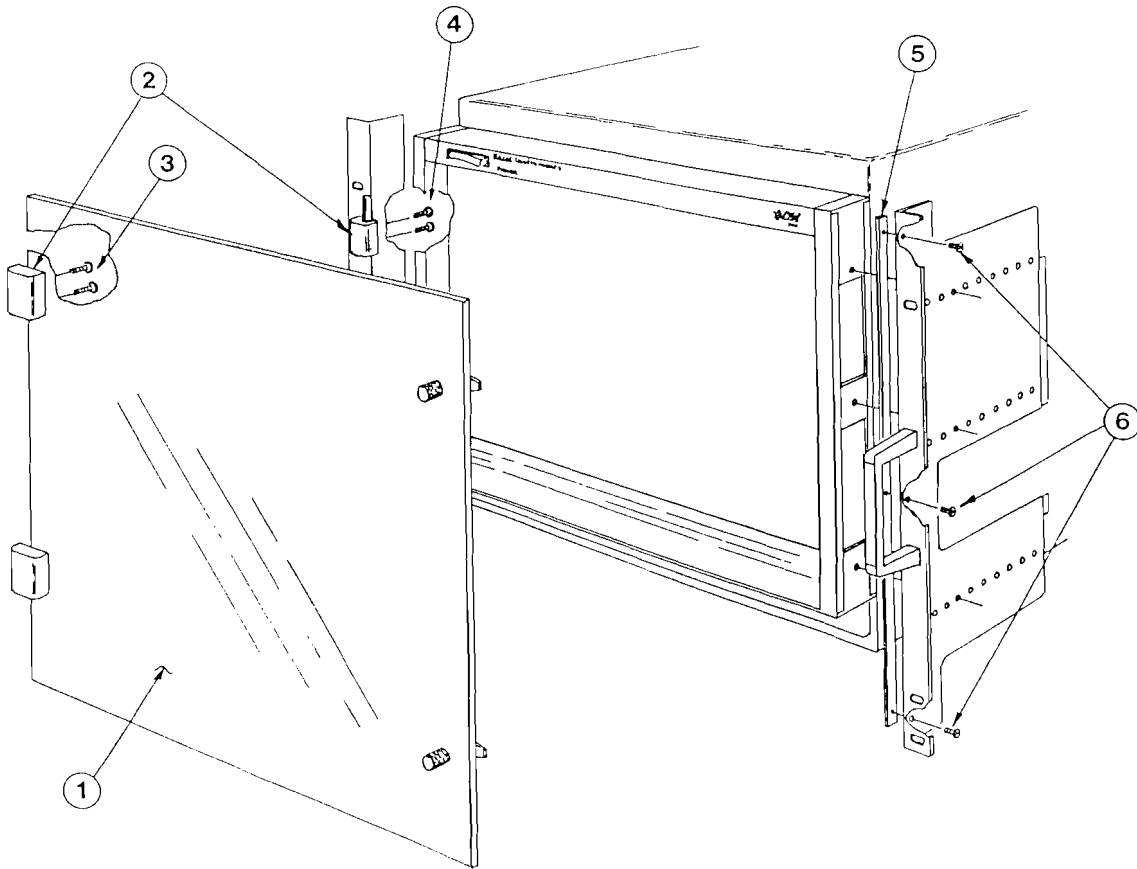
Figure 2-8 Installing Rack Mount Door
