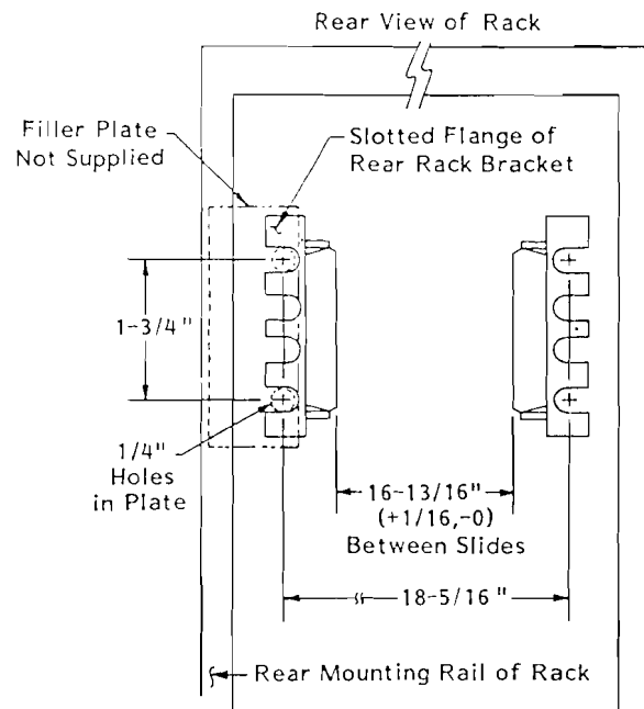
Figure 2-6 Rear End Slide Mount Rack Dimensions
