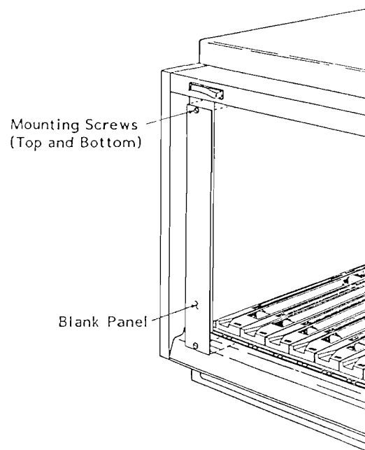
Figure 2-2 Blanking Panels
