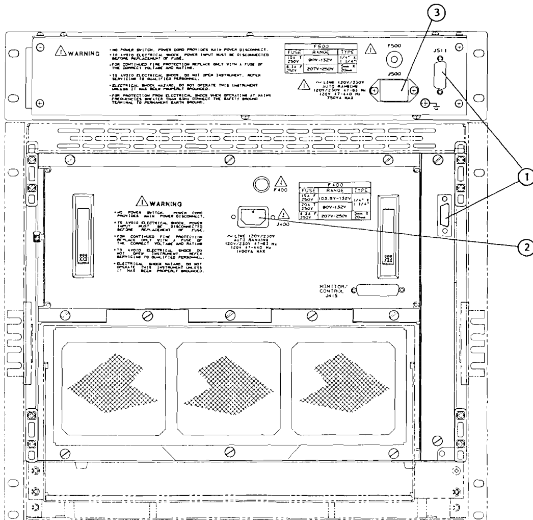
Figure 2-10 Connecting The Current Sharing Supply Option 53
