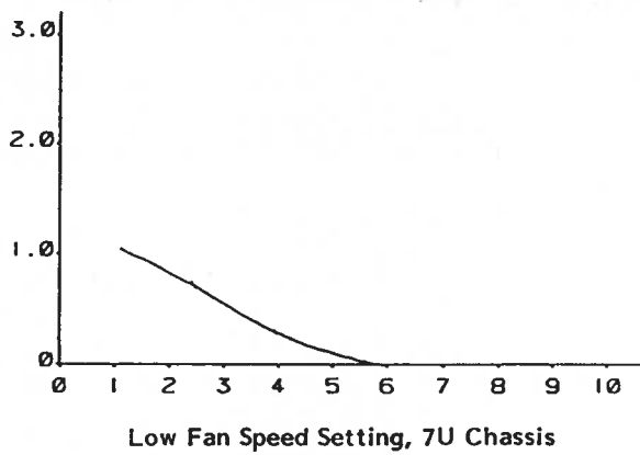
Figure A-1 Mainframe Worst Case Slot Cooling Curve
