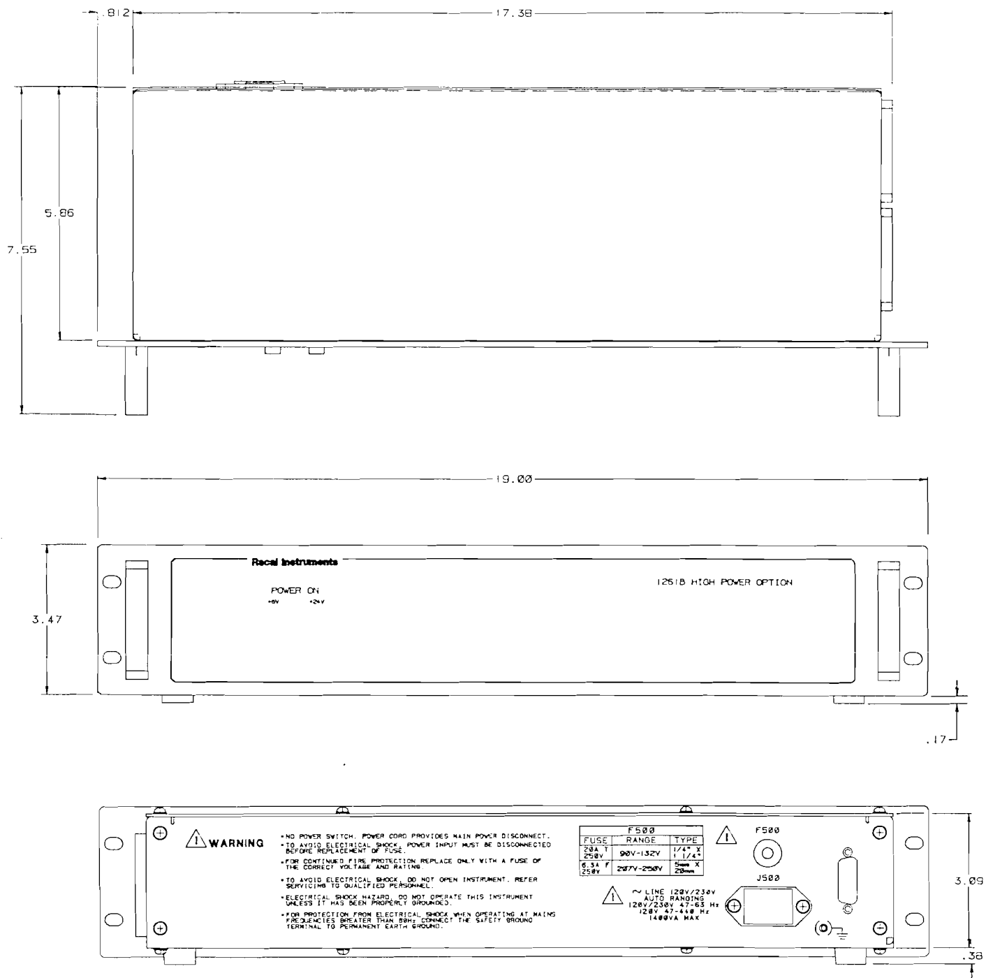
Figure A-7 Current Sharing Supply, Option 53 Views (For Use With 1261B Only)
