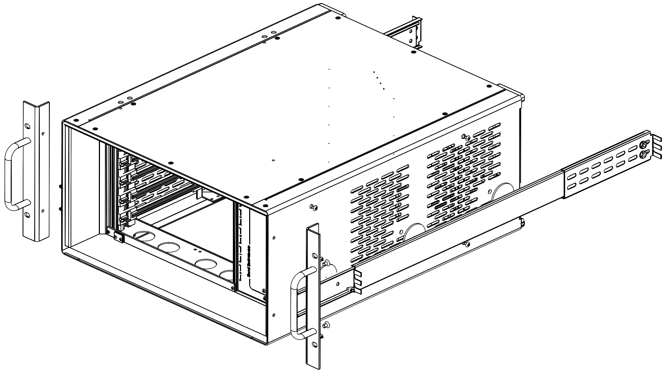
Figure 1-2, 1264C Rack Mount (5U Tall) Configuration
