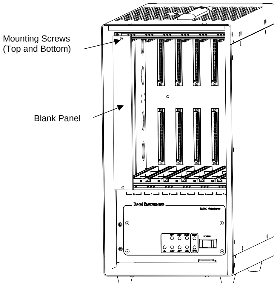
Figure 2-2, Blanking Panels
