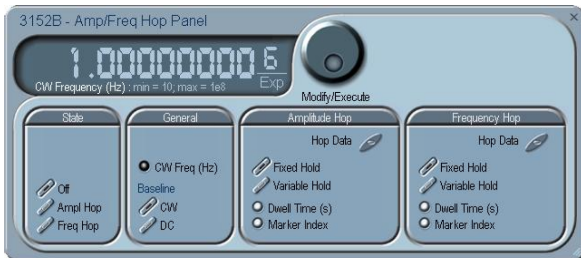
Figure 4-18, Amp/Freq Hop Panel
