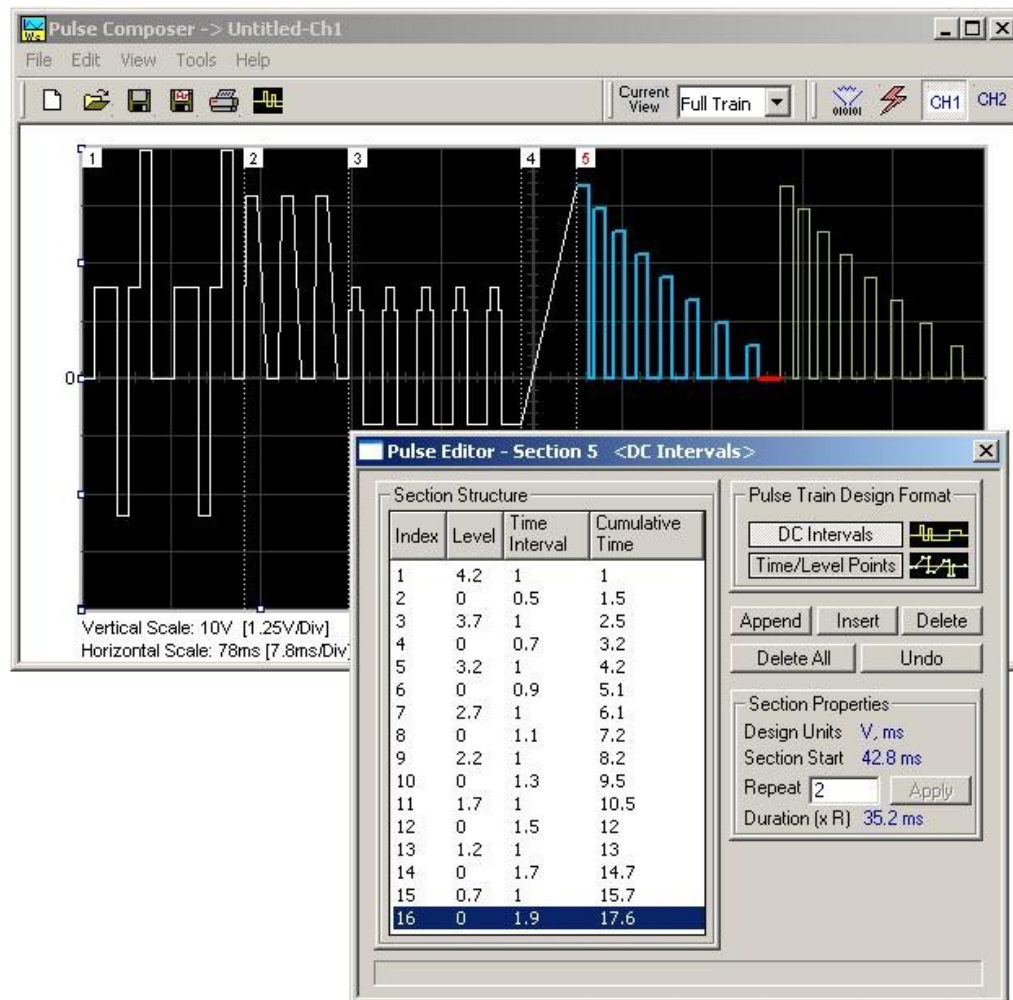
Figure 4-55, Building Section 5 of the Pulse Example
