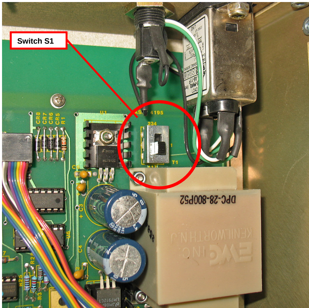
Figure 2-1. Switch S1 – Input Voltage Setting
