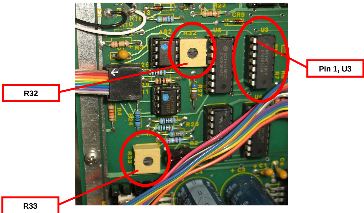
Figure 3-1. Calibration Adjustments
