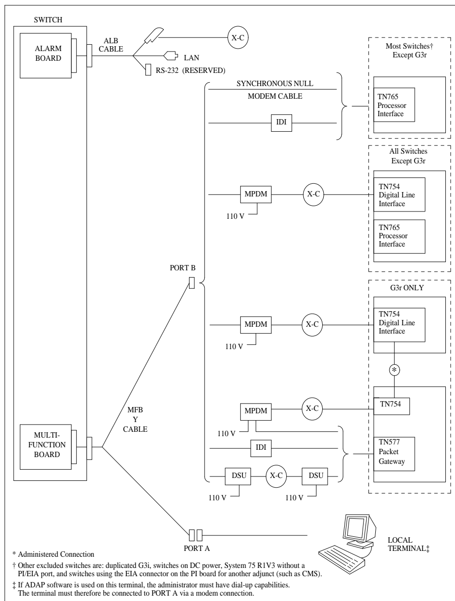
Figure 1-1. DEFINITY AUDIX System Connectivity Diagram — CL Mode
