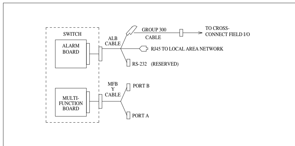
Figure 2-4. Alarm Board Cable Connections
