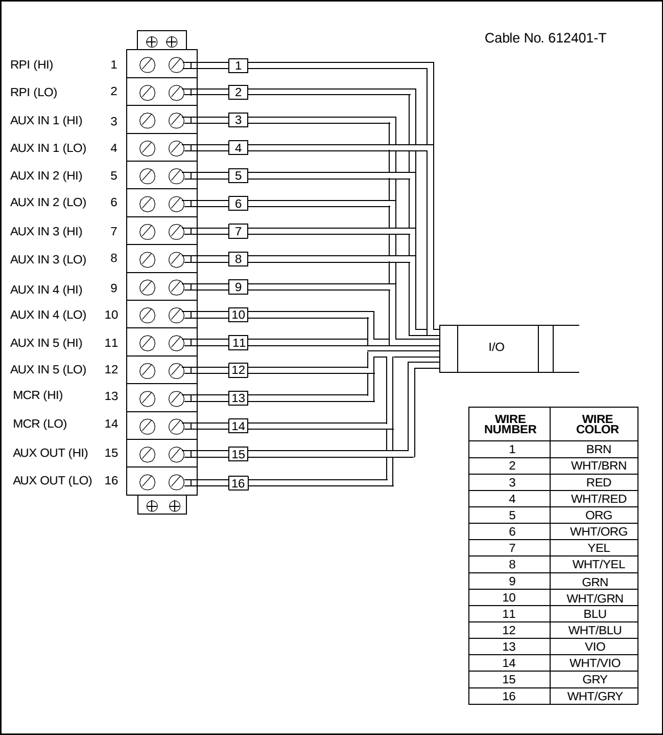
Figure 4.3 – Terminal Block Connections for Drive I/O
