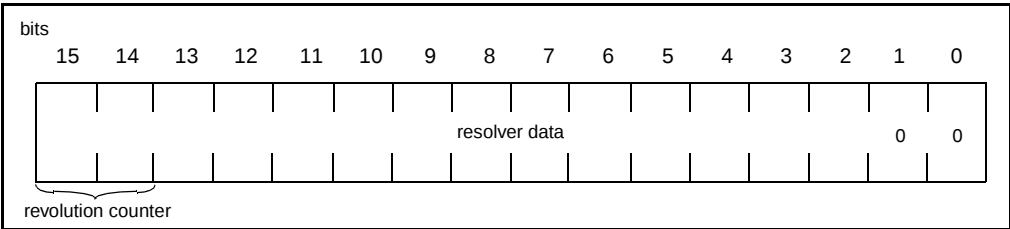
Figure 3.1 – Resolver Data Format (12-Bit Mode)
