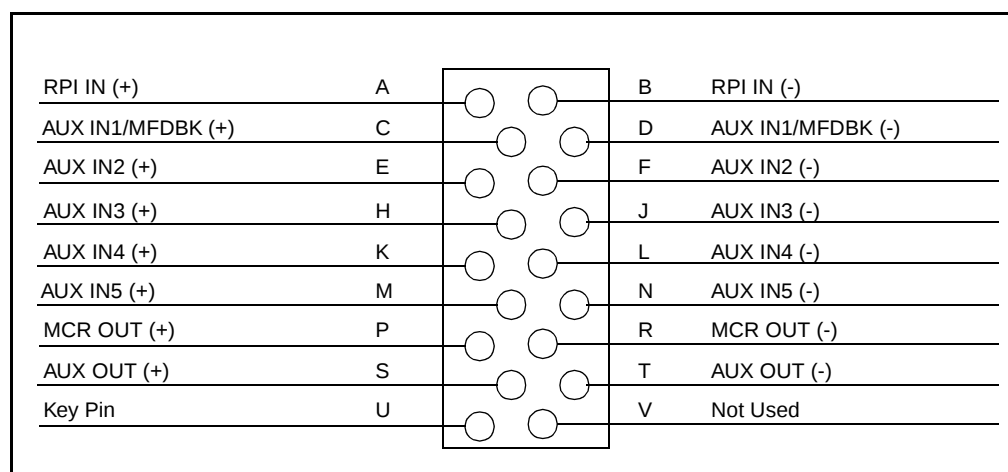
Figure 2.7 shows the auxiliary input interface circuit.
