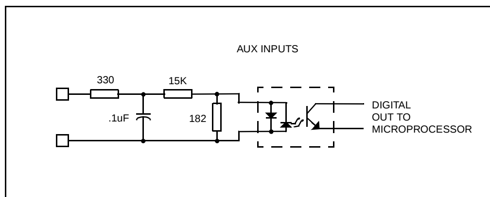
Figure 2.7 shows the auxiliary input interface circuit.
