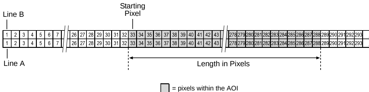
Fig. 42: Area of Interest
