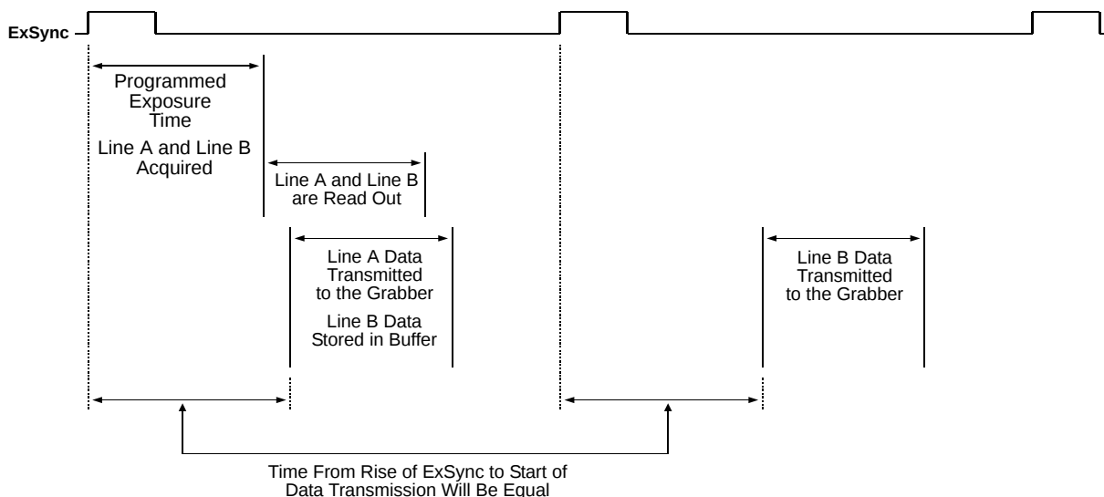
Fig. 15: Dual Line Acquisition with ExSync Programmable Exposure and Line A First
