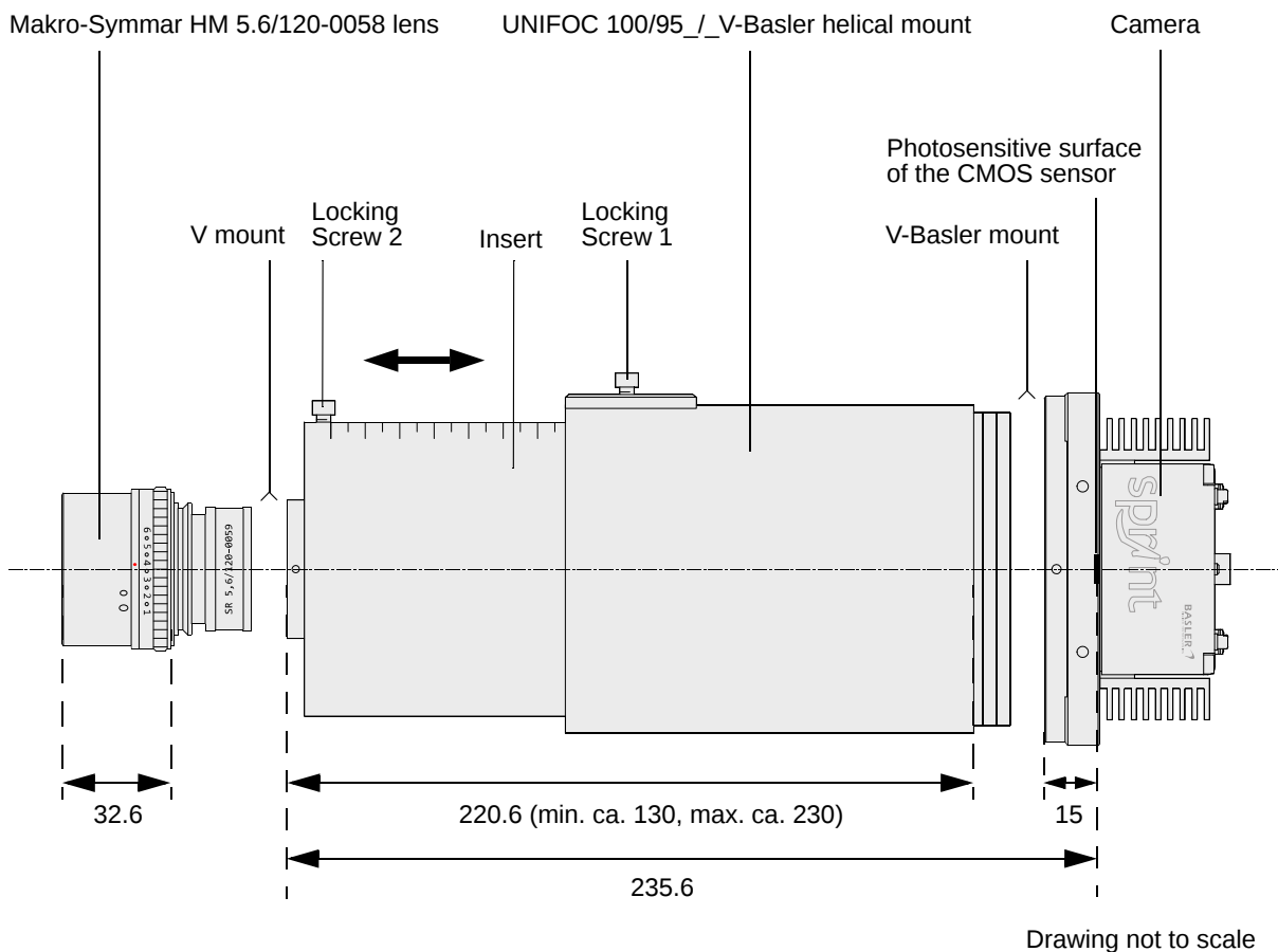
Fig. 2: Using the UNIFOC 100/05_/_V-Basler Helical Mount (Distances in mm)
