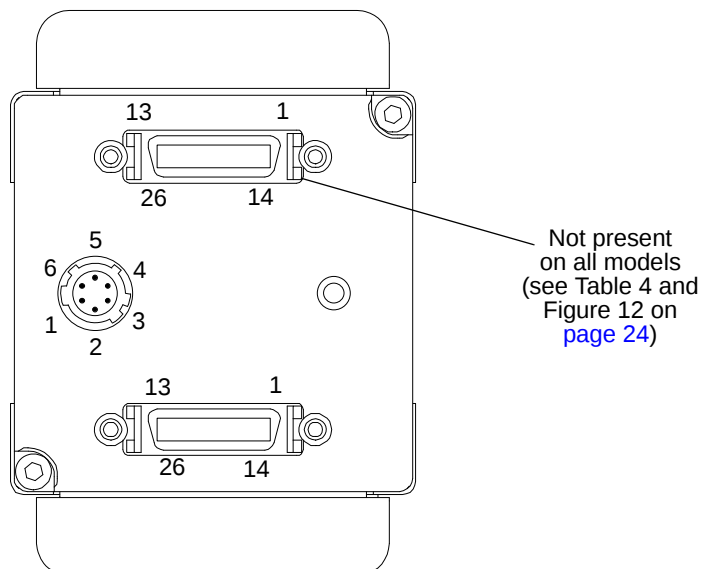
Fig. 13: Pin Numbering (2k and 4k cameras; 8k cameras are analogous)
