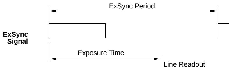
Fig. 29: ExSync Programmable Mode
