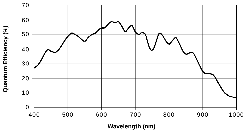
Fig. 4: Camera Spectral Response
