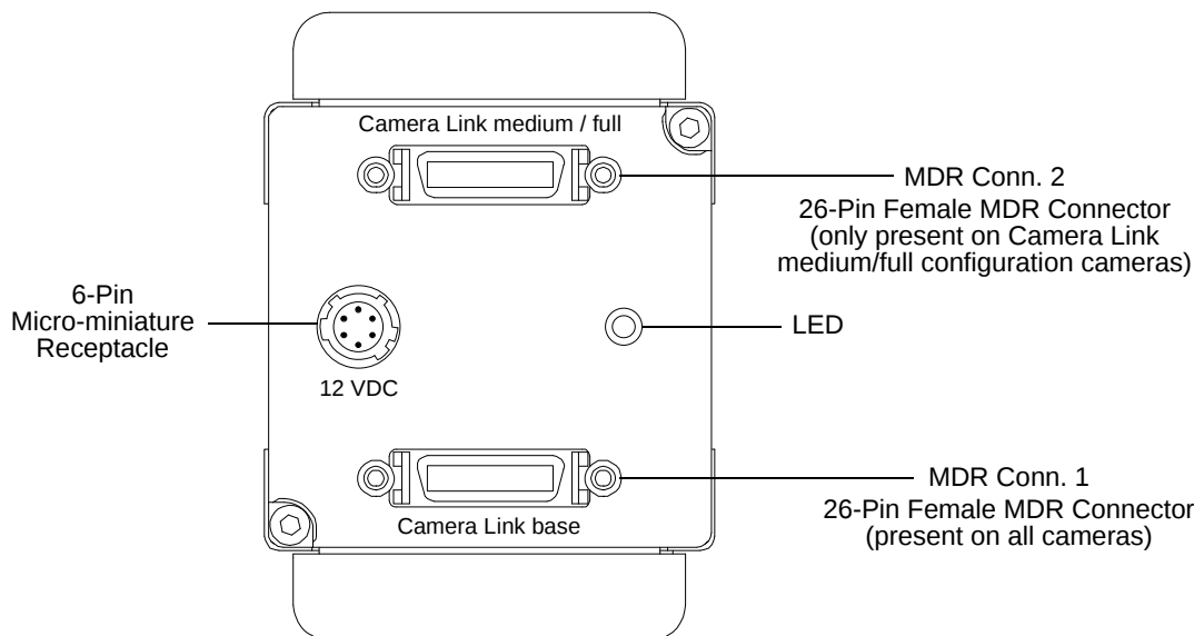
Fig. 12: Connectors and LED (2k and 4k cameras; 8k cameras are analogous)
