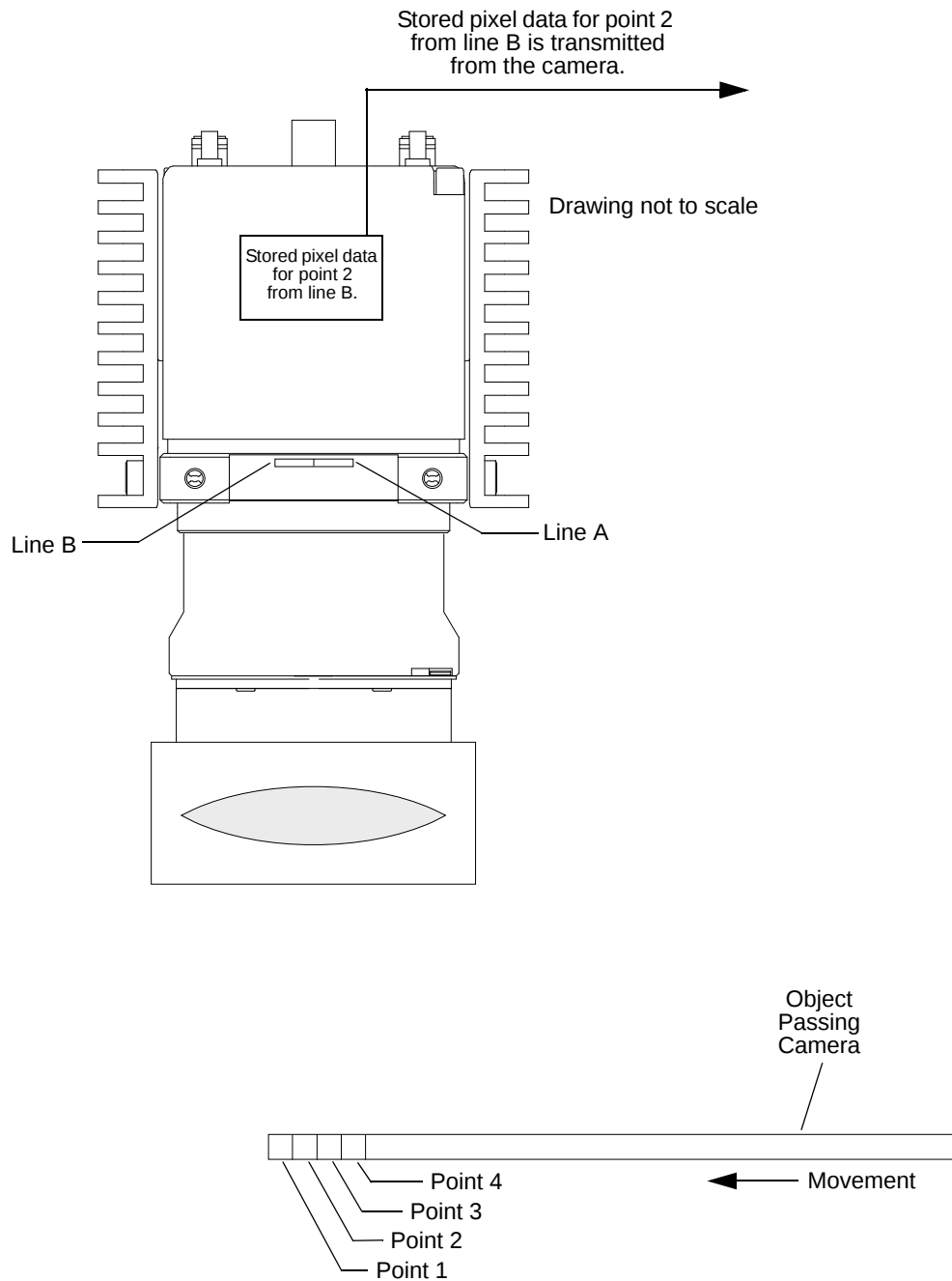
Fig. 17: Dual Line Acquisition - ExSync Cycle 2
