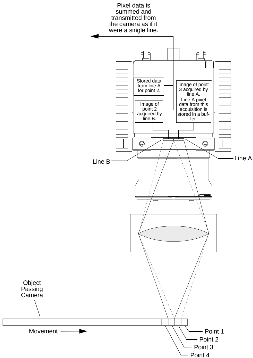
Fig. 23: Time Delayed Line Summing - Acquisition Three
