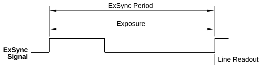
Fig. 27: ExSync Edge Controlled Mode
