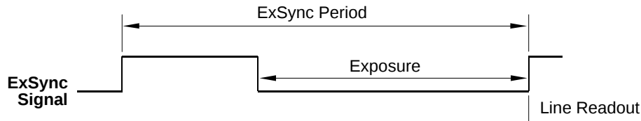
Fig. 28: ExSync Level Controlled Mode
