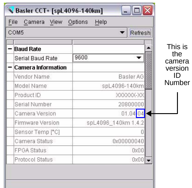
Fig. 1: CCT+ Window
