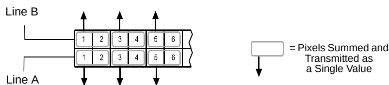
Fig. 25: Horizontal Binning
