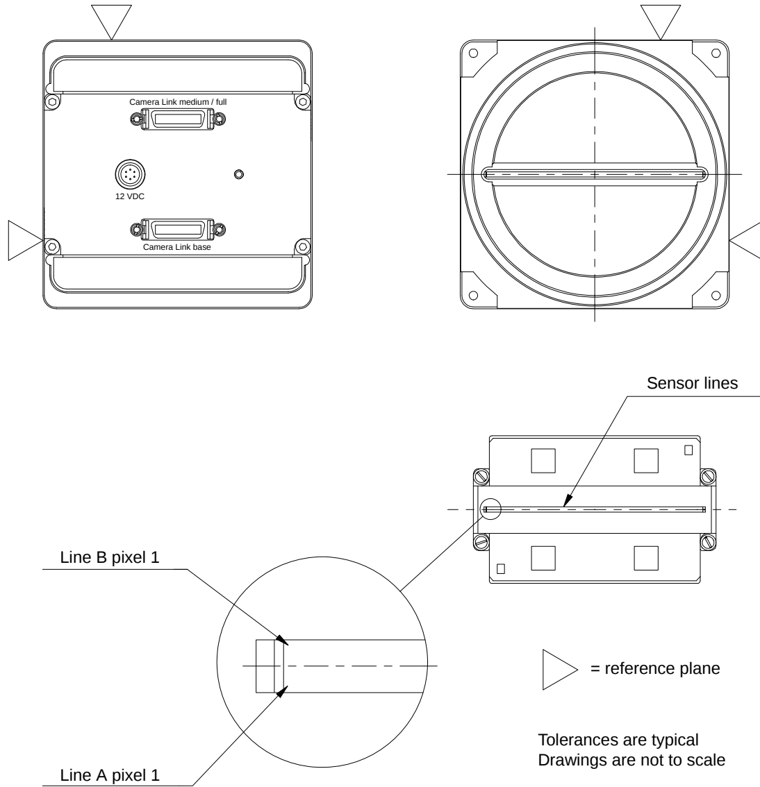
Fig. 11: Sensor Line Location (8k Cameras)
