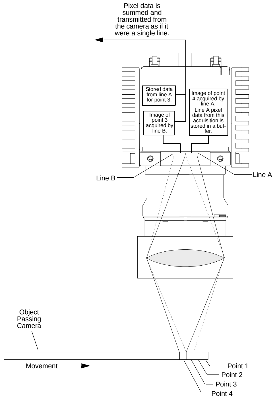
Fig. 24: Time Delayed Line Summing - Acquisition Four
