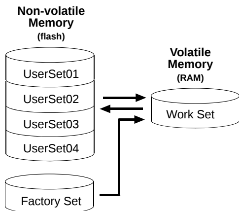
Fig. 49: Configuration Sets
