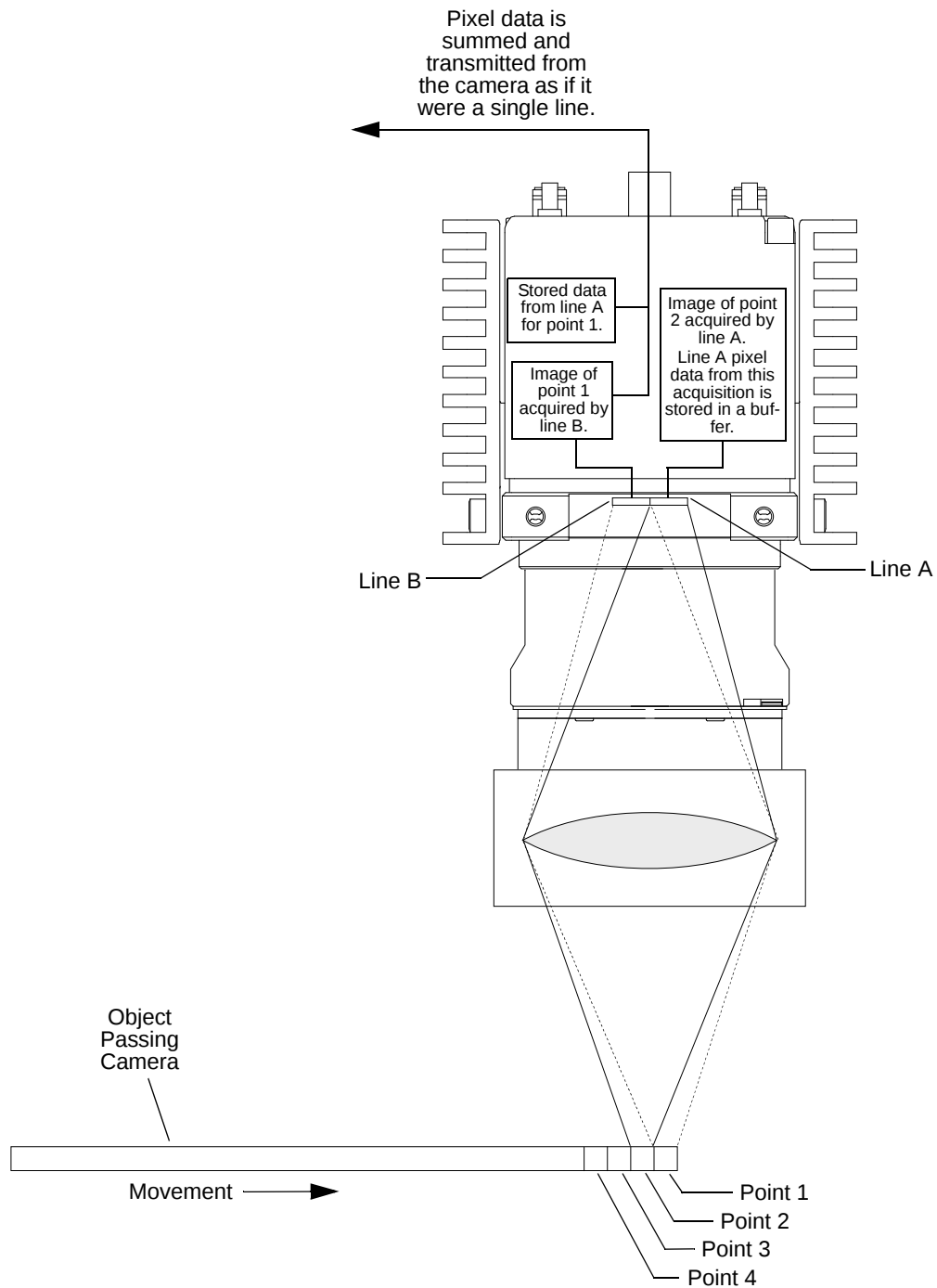
Fig. 22: Time Delayed Line Summing - Acquisition Two
