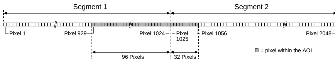
Fig. 34: AOI Falling Across Segments - Horizontal Binning Enabled
