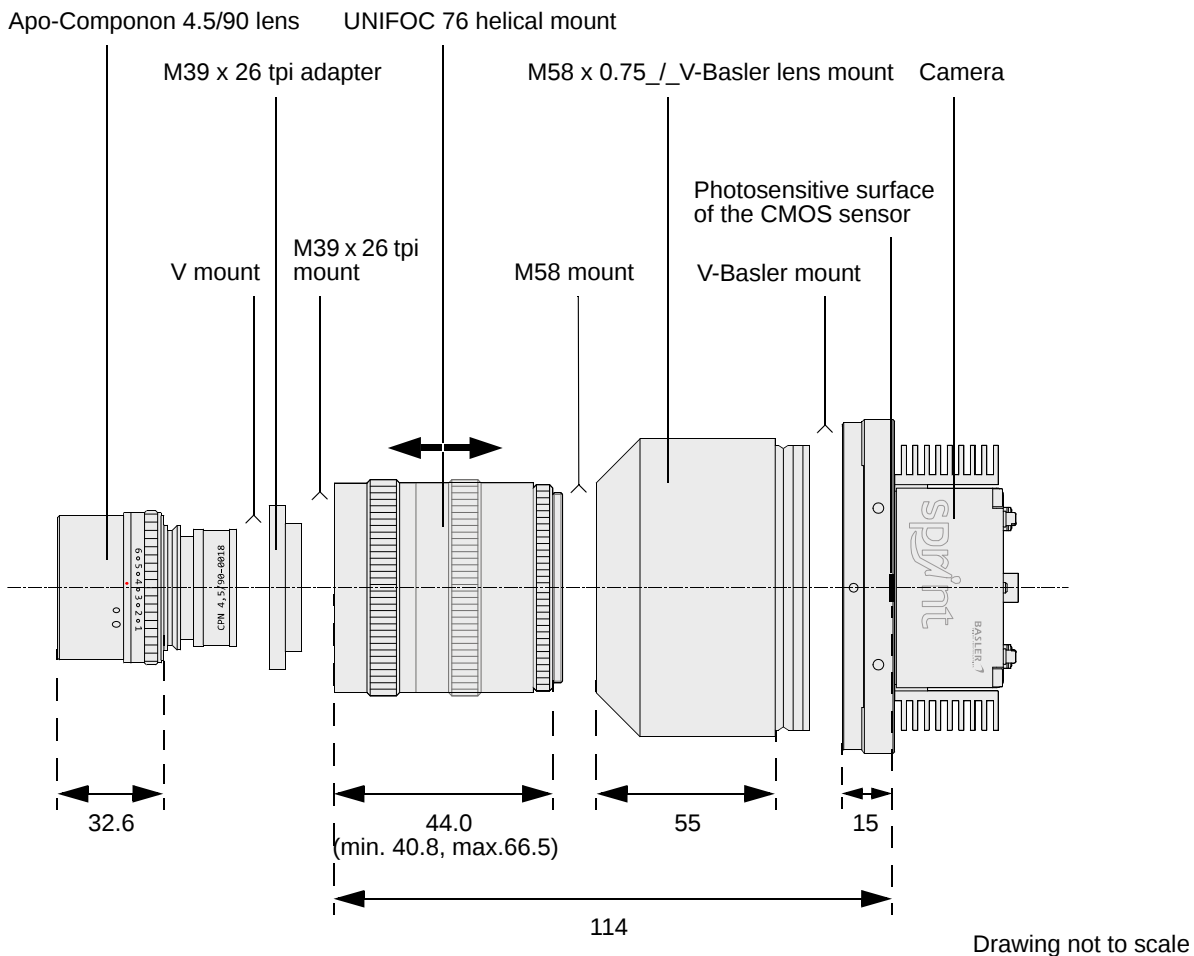
Fig. 3: Using the M58 x 0.75 / V-Basler Lens Mount (Distances in mm)
