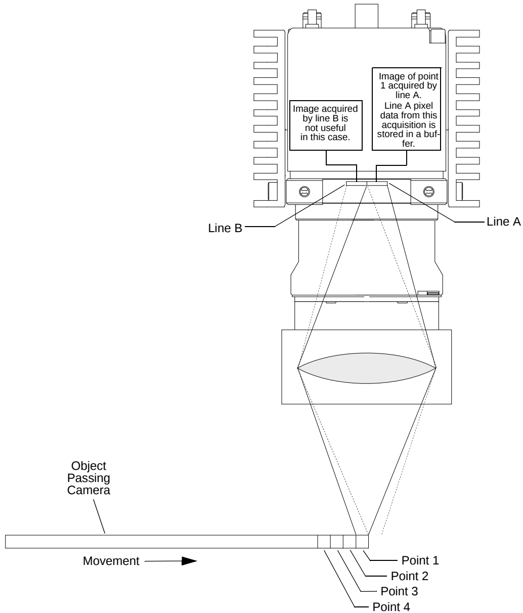
Fig. 21: Time Delayed Line Summing - Acquisition One
