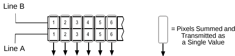
Fig. 20: Vertical Binning
