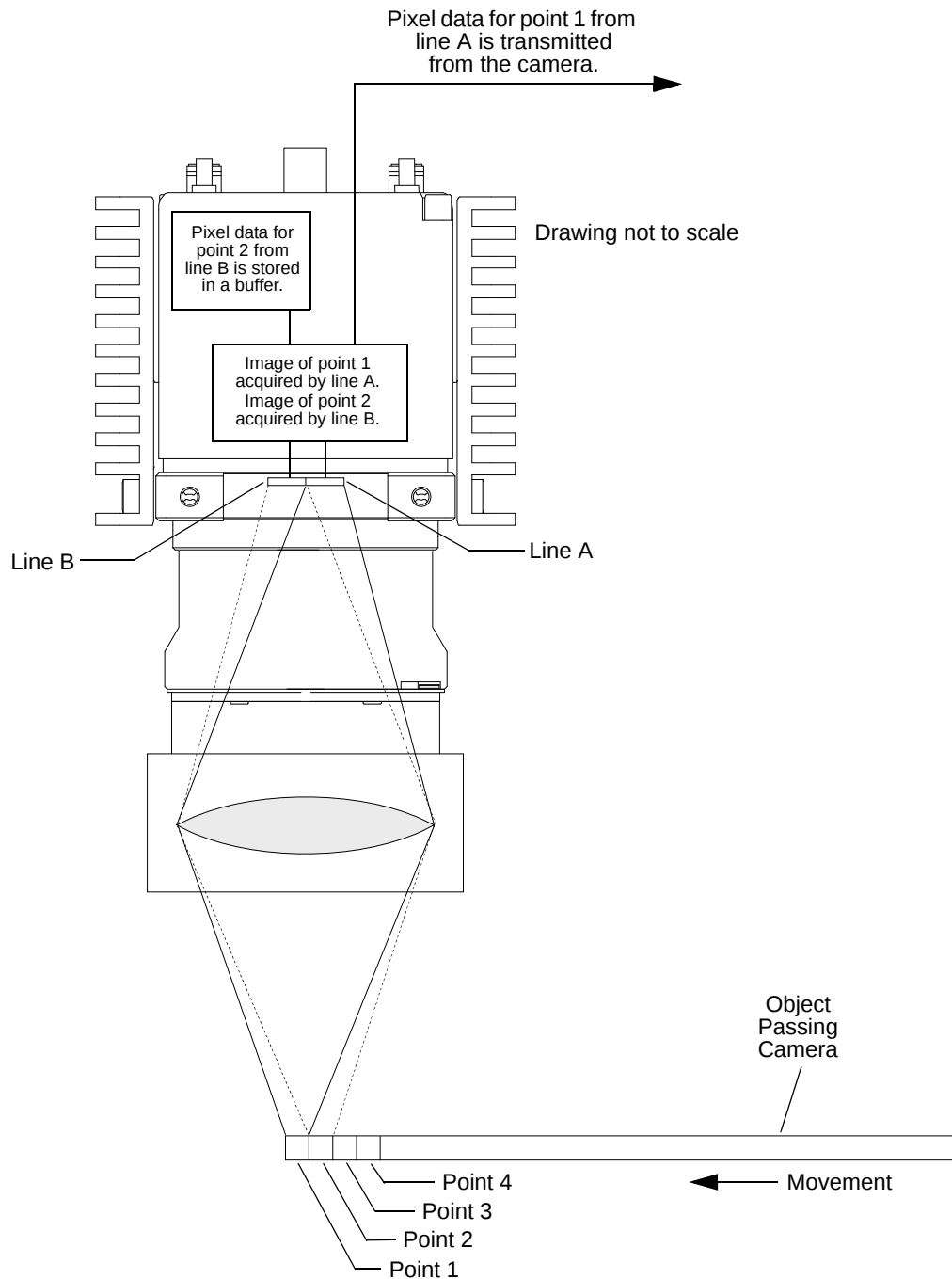
Fig. 16: Dual Line Acquisition - ExSync Cycle 1
