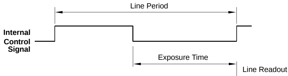
Fig. 31: Free Run, Programmable Mode
