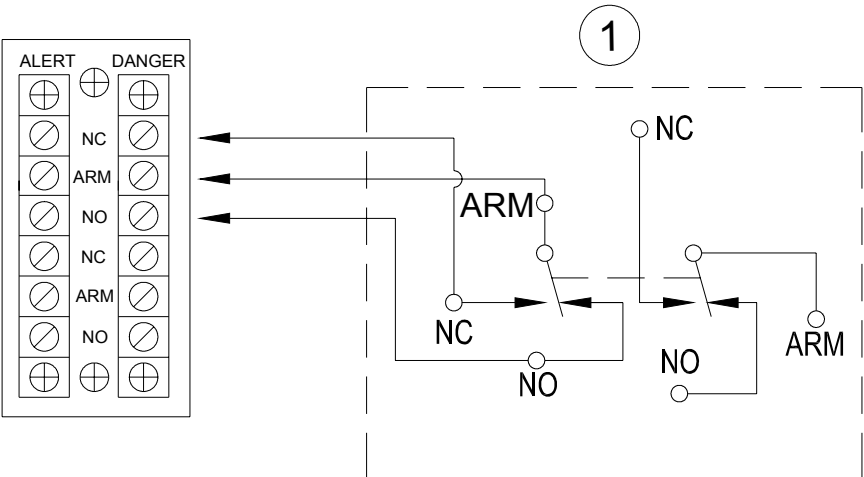
Figure 2 Normally Energized
