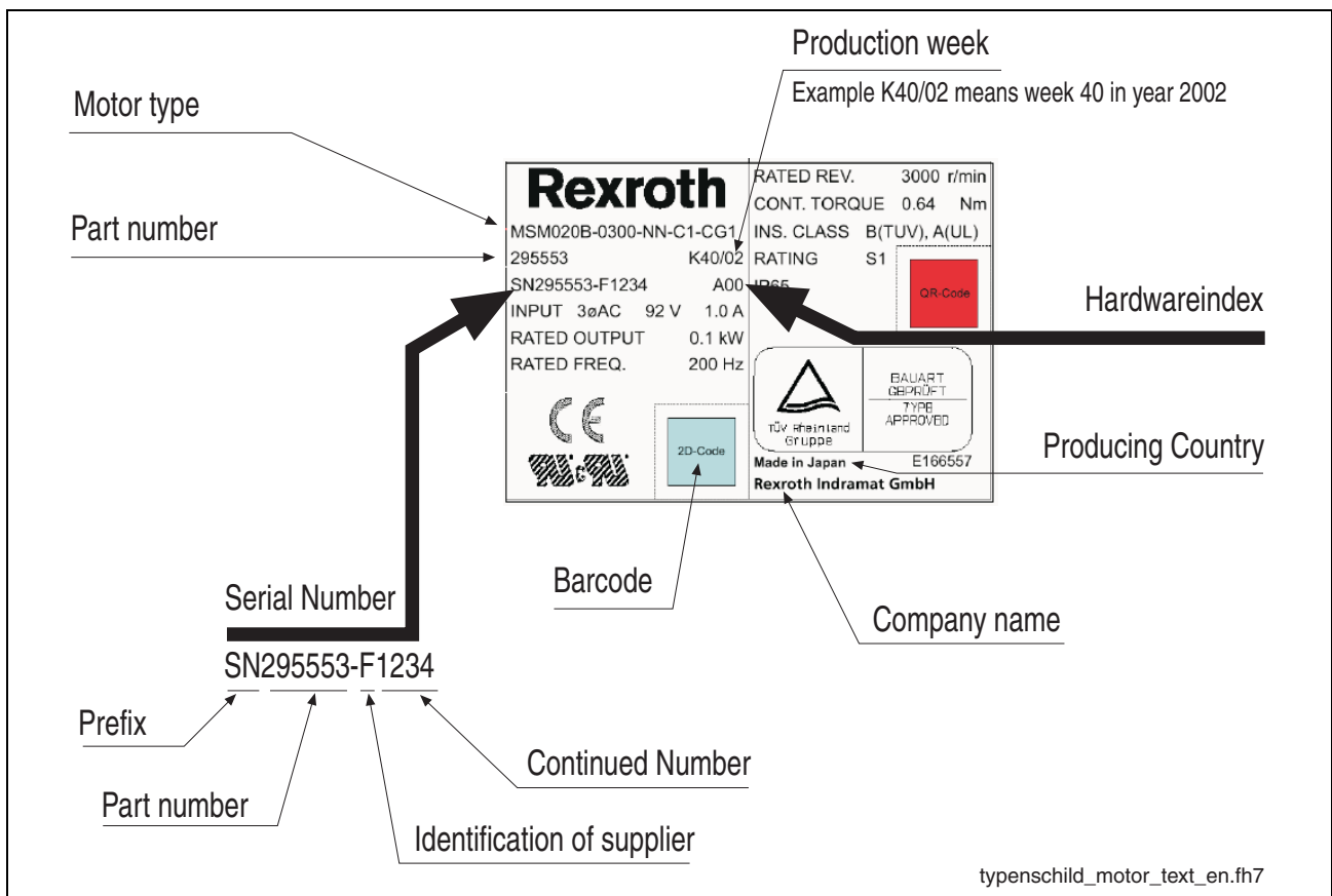
Fig. 9-5: Motor type plate
