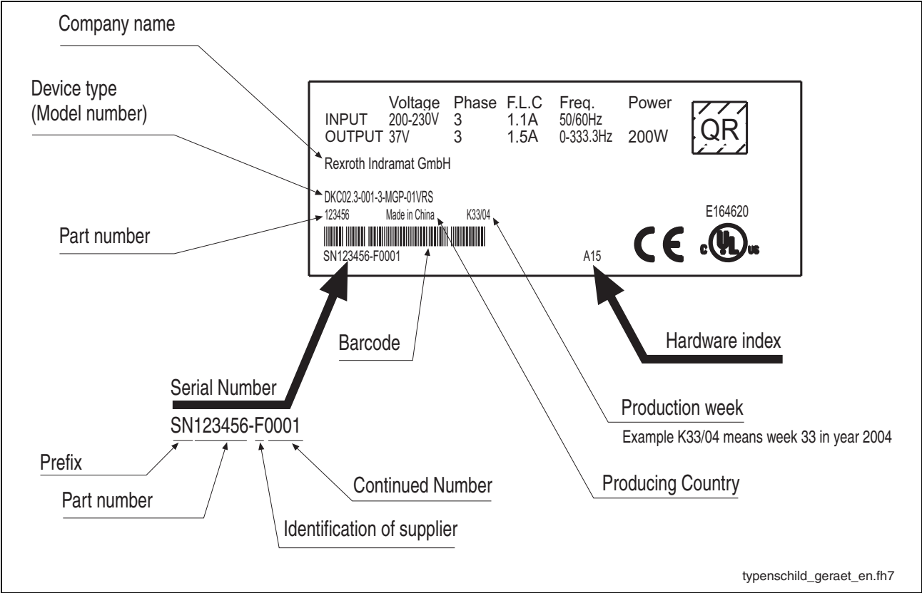
Fig. 9-2: Type plate 1
