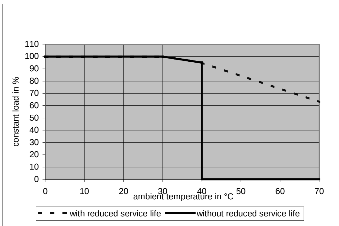
Fig. 8-11: MSM020B utilization depending on the ambient temperature
