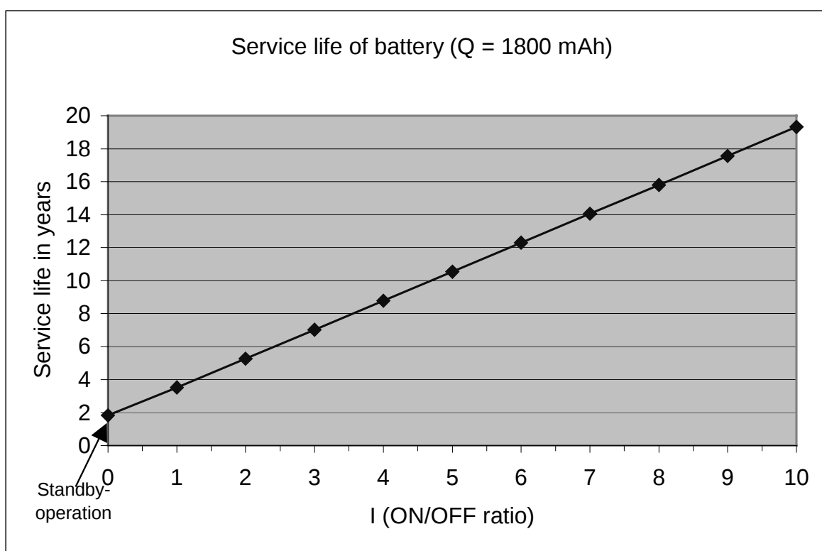
Fig. 8-54: Service life of battery
