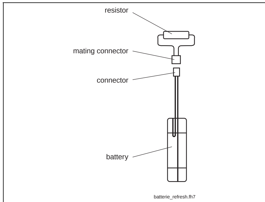
Fig. 8-55: Battery refreshing
