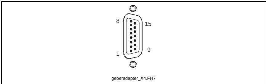
Fig. 10-20: Connector X4
