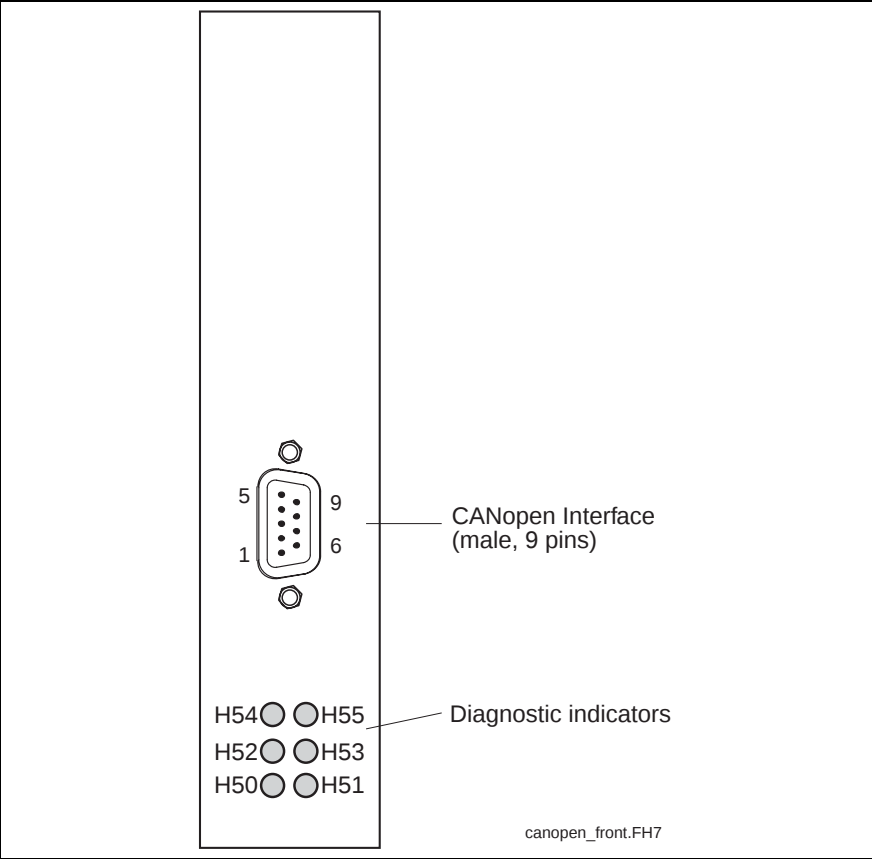
Fig. 5-87: View of interface to master communication
