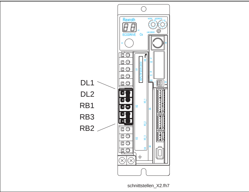
Fig. 5-9: Terminal connector X2
