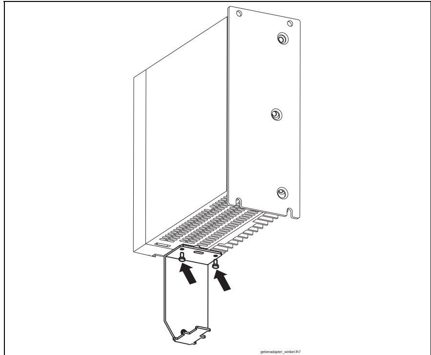
Fig. 10-16: Angle plate
