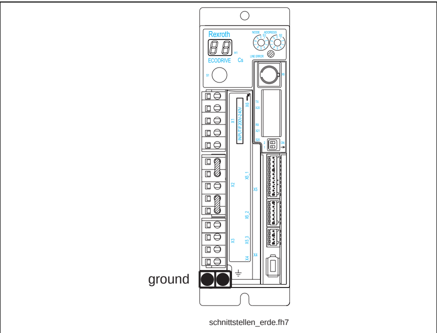
Fig. 5-18: Ground connection
