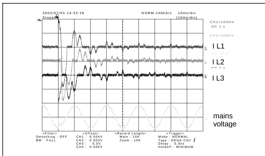
Fig. 6-12: Currents I L1, I L2, I L3 and mains voltage or transformer output when switching on (time basis: T = 10 \text{ ms/div} )
