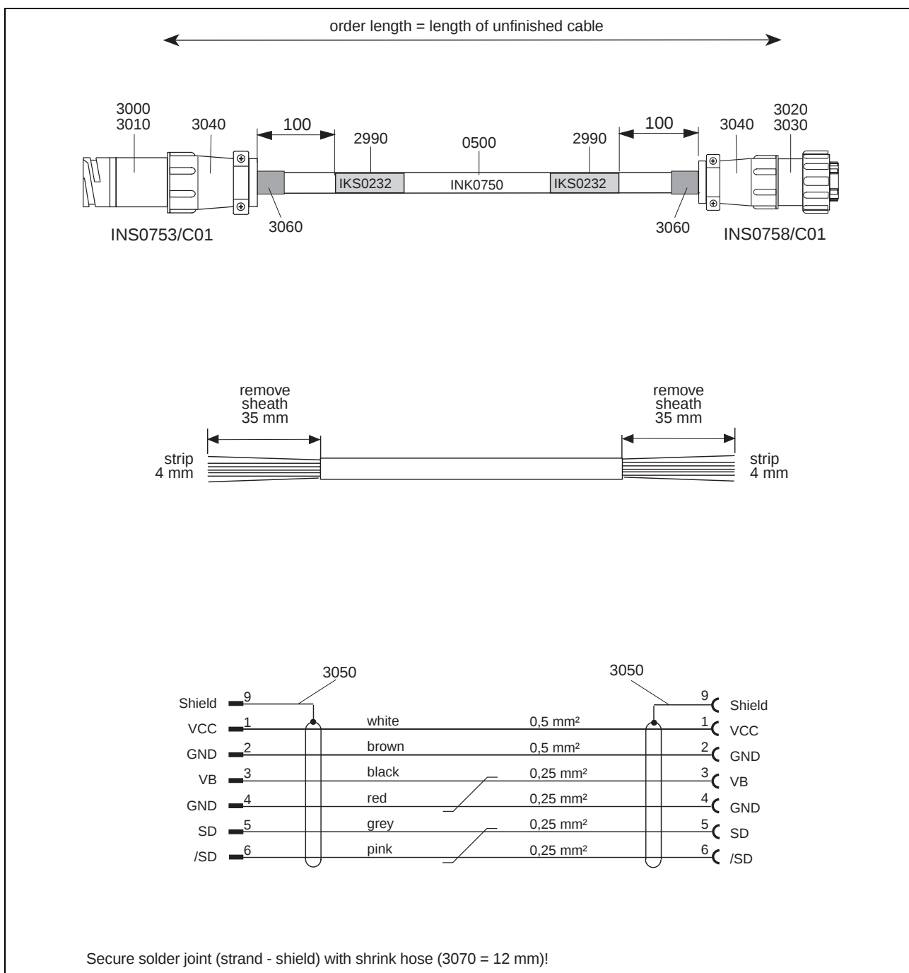
Fig. 10-4: Encoder extension cable IKS0232
