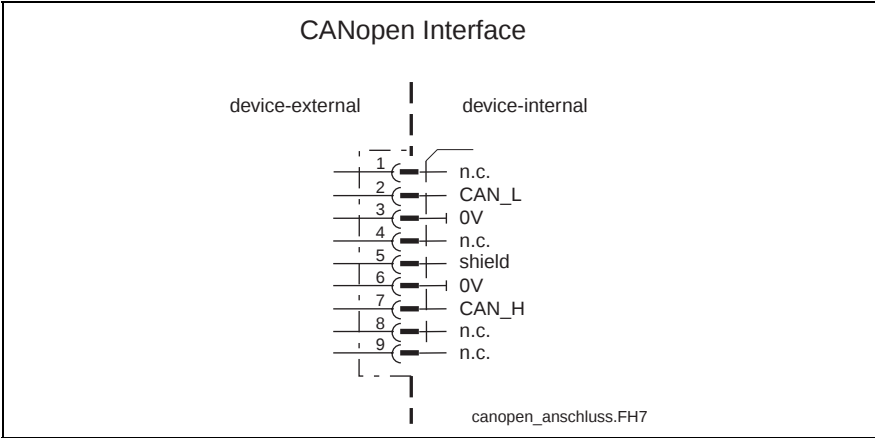
Fig. 5-90: Connection
