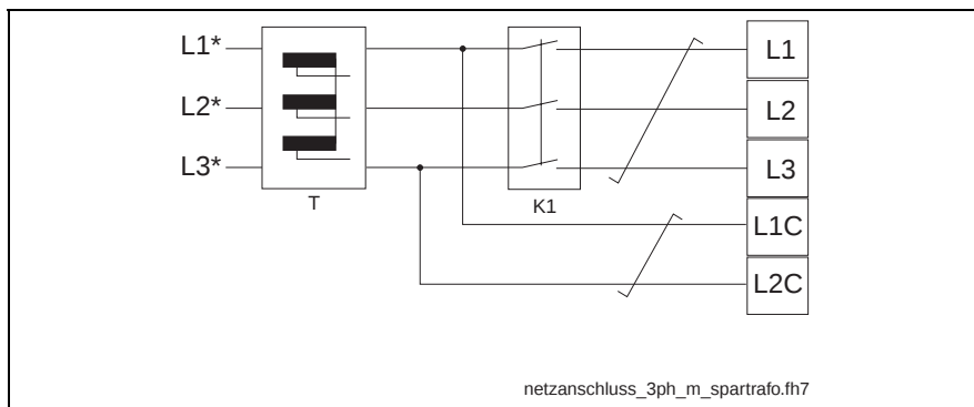
Connection to Drive Controller
