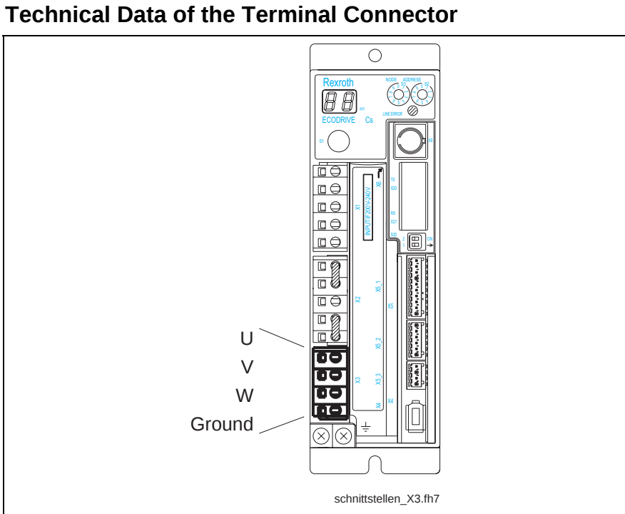
Fig. 5-15: Terminal connector X3
