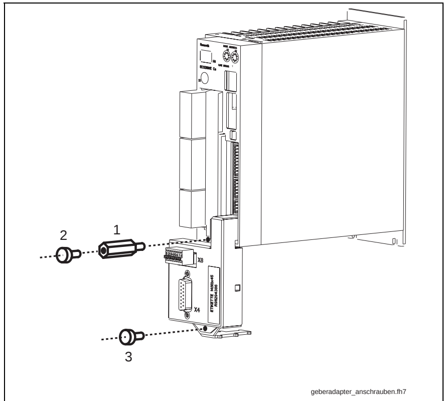
Fig. 10-18: Screw on the encoder adapter
