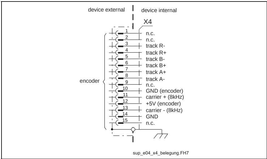
Fig. 10-23: Connection
