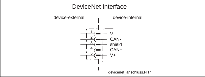
Fig. 5-78: Connection
