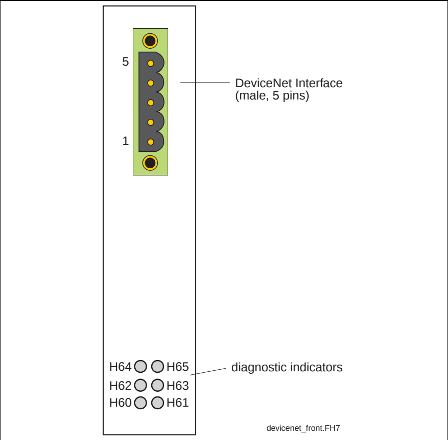
Fig. 5-75: View of interface to master communication
