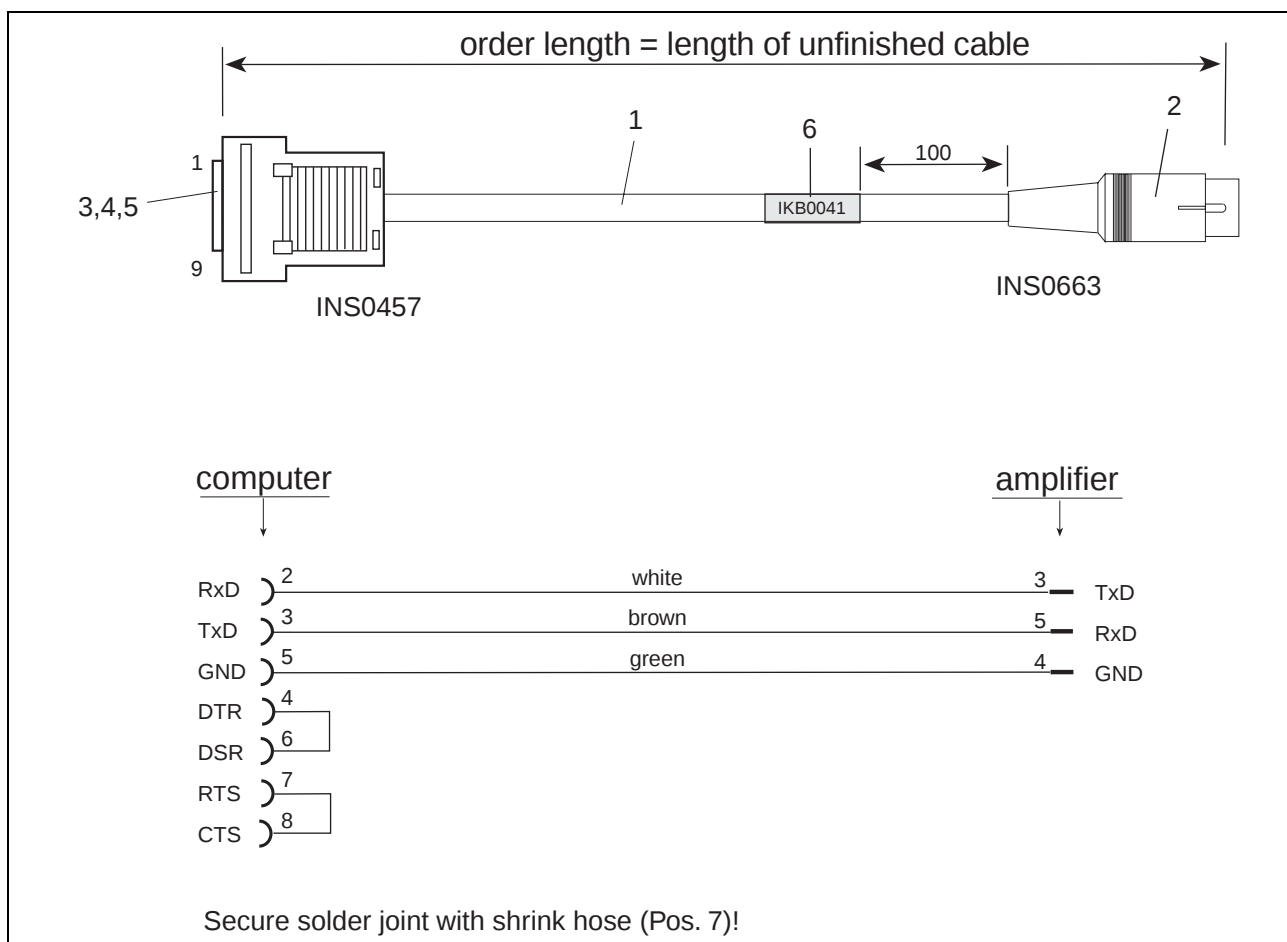
Fig. 10-6: RS232 cable
