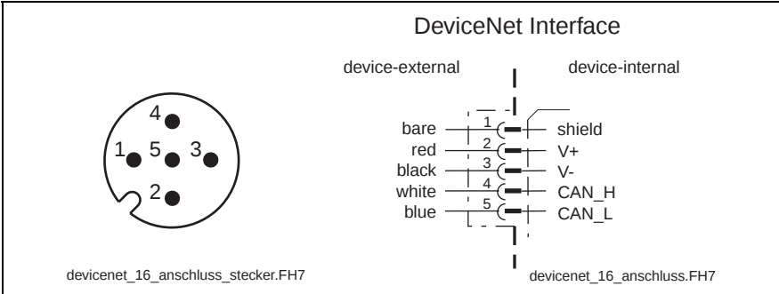
Fig. 5-84: Connection
