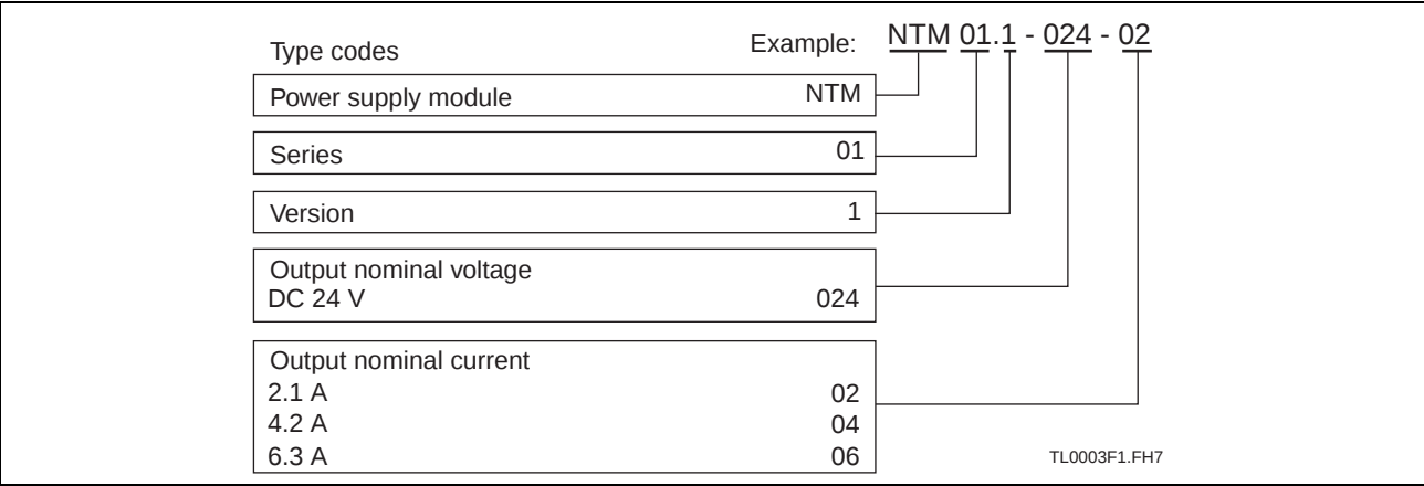
Fig. 10-42: Type code
