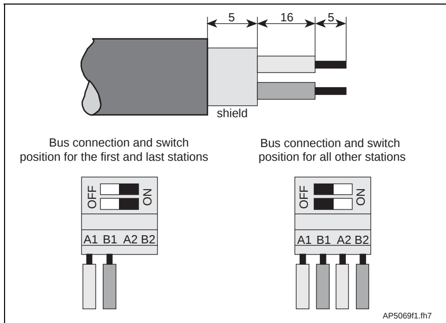
Fig. 5-70: Preparing a cable for connecting a bus connector
