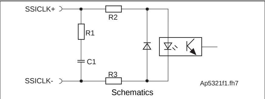
Fig. 5-57: Differential input circuit
