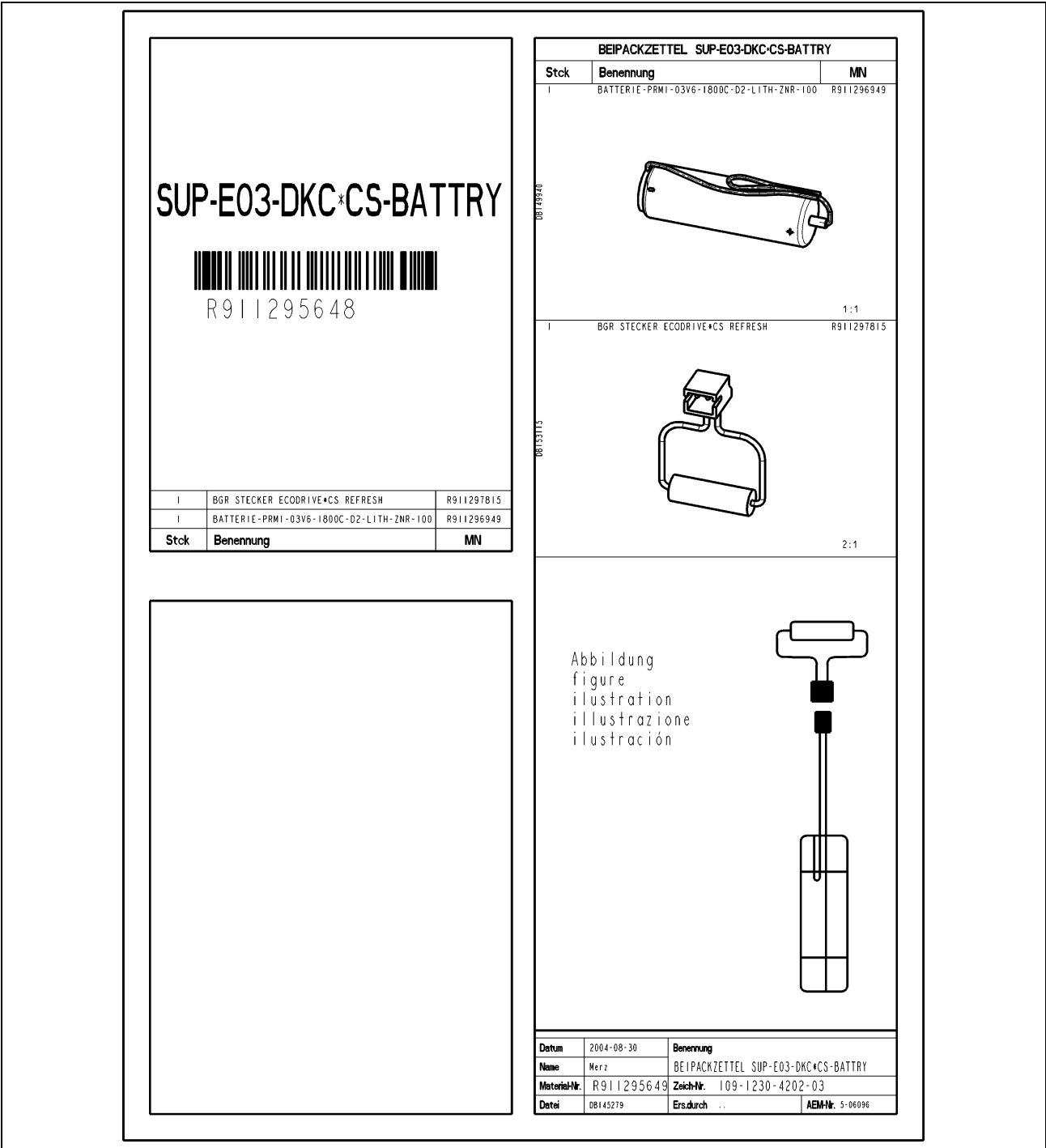
Fig. 10-13: SUP-E03-DKC*CS-BATTERY
