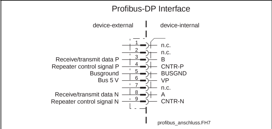
Fig. 5-67: Connection
