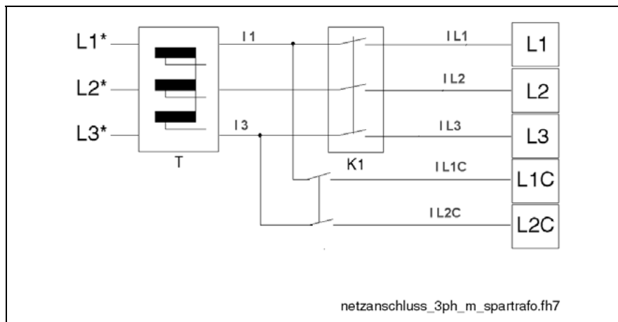
Fig. 6-11: Test setup for current measurement with three-phase connection ( U = 3 \times 230 \text{ V} )
