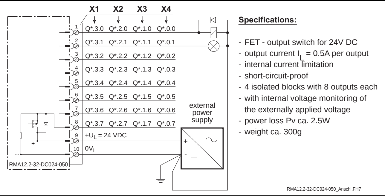
Figure 8-21: Wiring diagram of RMA12.2-DC024-050
