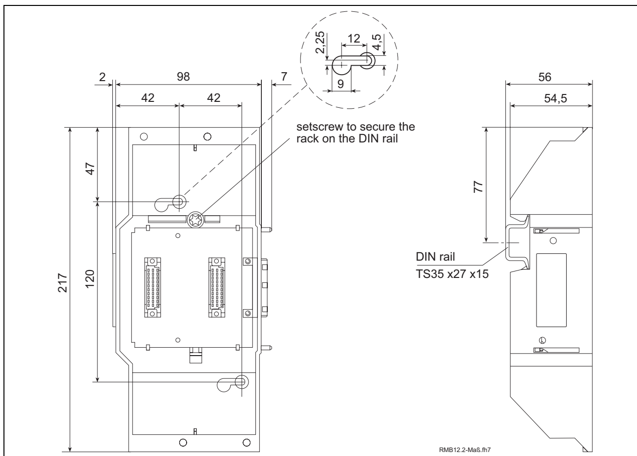
Figure 1-3: RMB12.2-02 base rack
