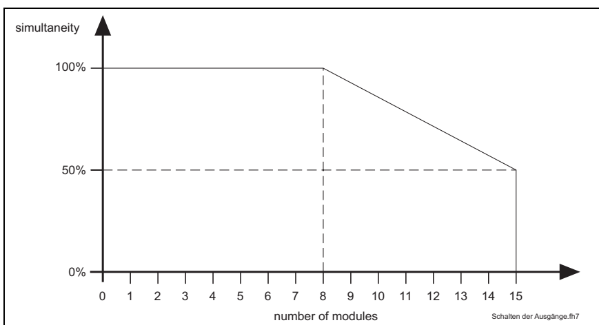
Figure 12-41: Maximum number of outputs that can be switched simultaneously.
