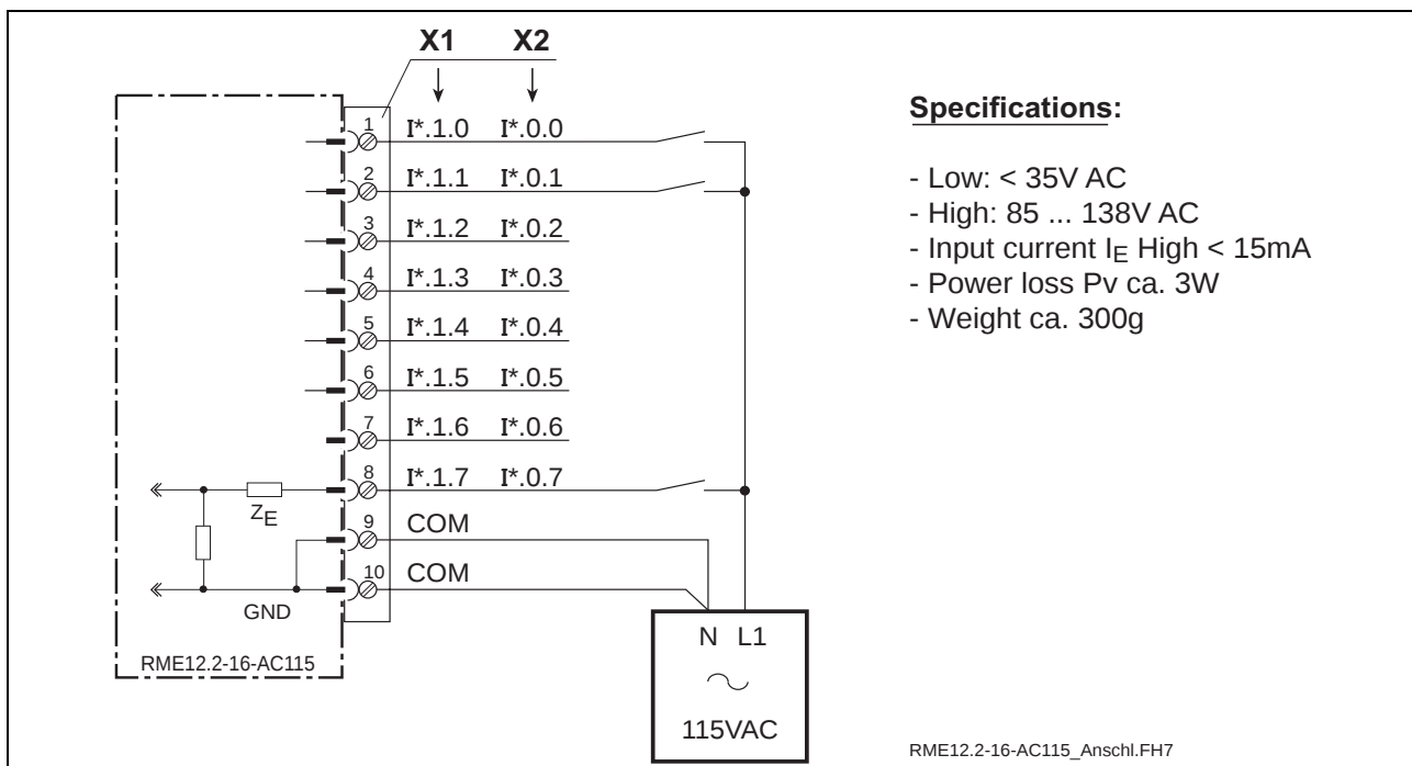
Figure 6-17: Wiring diagram of RME12.2-16-AC115
