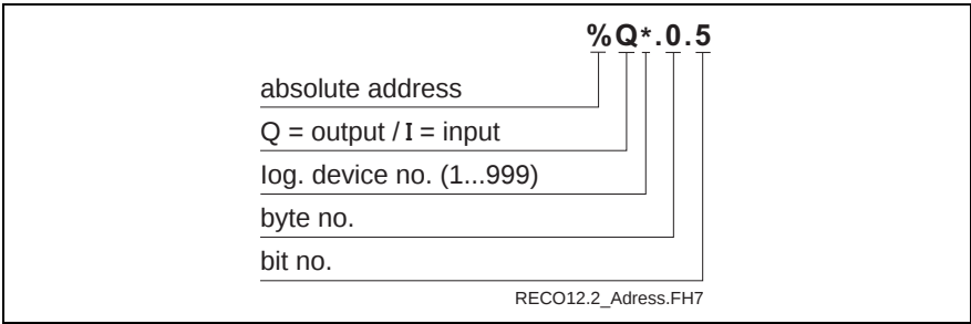
Figure 2-6: Typical address selection for an output module
