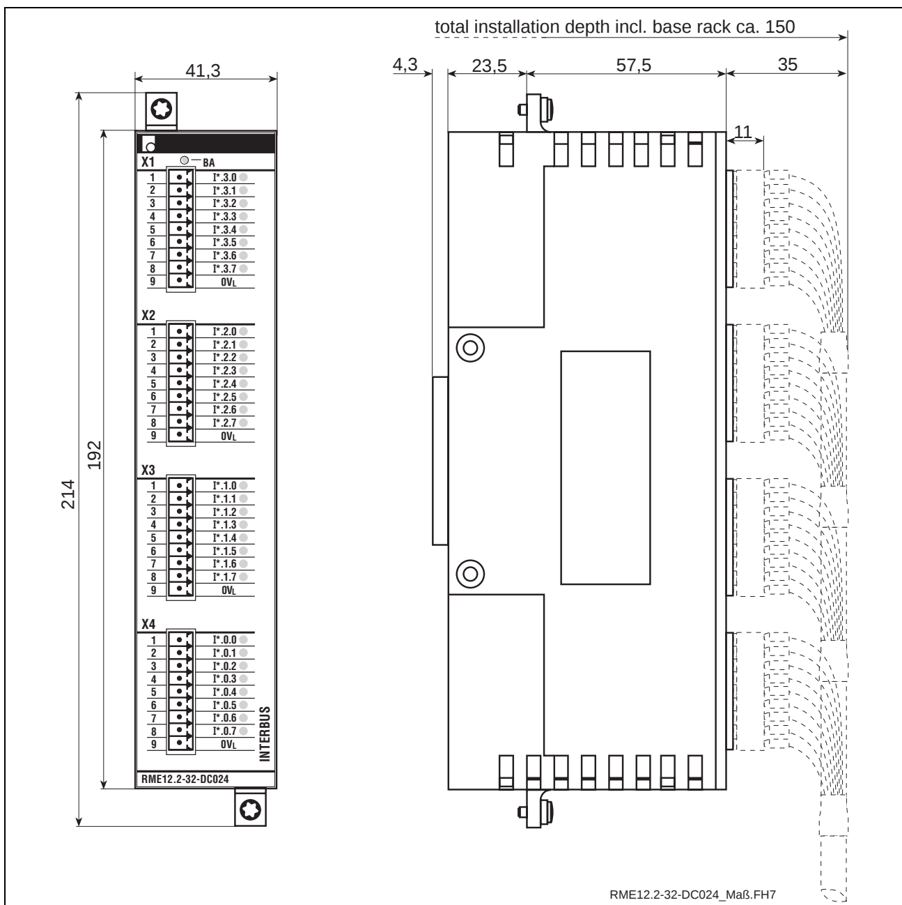
Figure 5-14: Mounting dimensions of RME12.2-32-DC024
