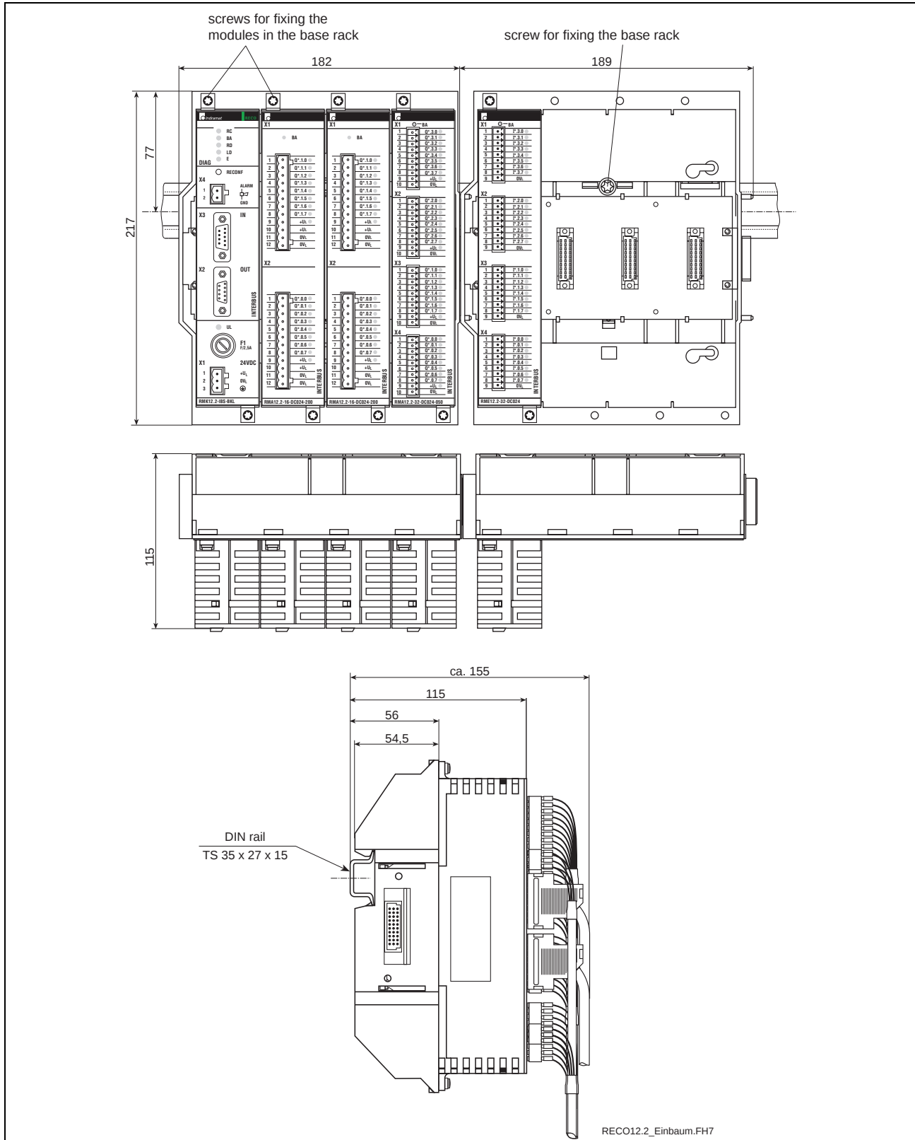
Figure 1-2: Mounting dimensions of the RECO12.2 unit
