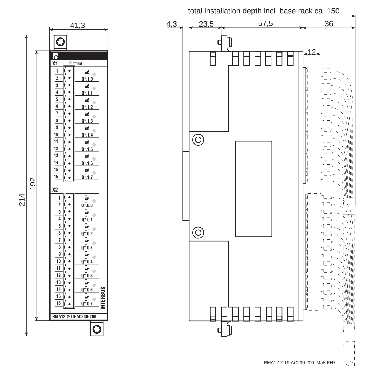
Figure 9-22: Mounting dimensions of RMA12.2-16-AC230-200
