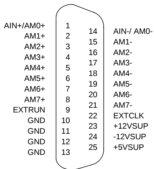
Figure A-2. D-SUB Connector Configuration
