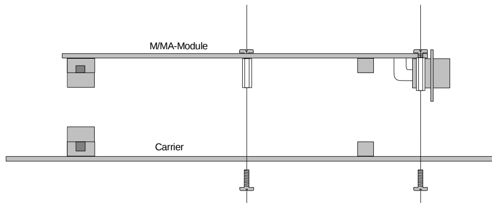
Figure 1. M-MODULE Installation
