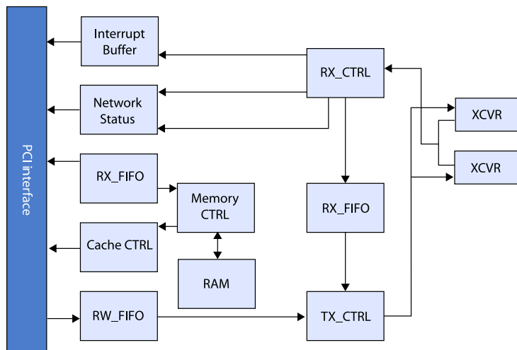
Figure 1: SCRAMNet Block Diagram
