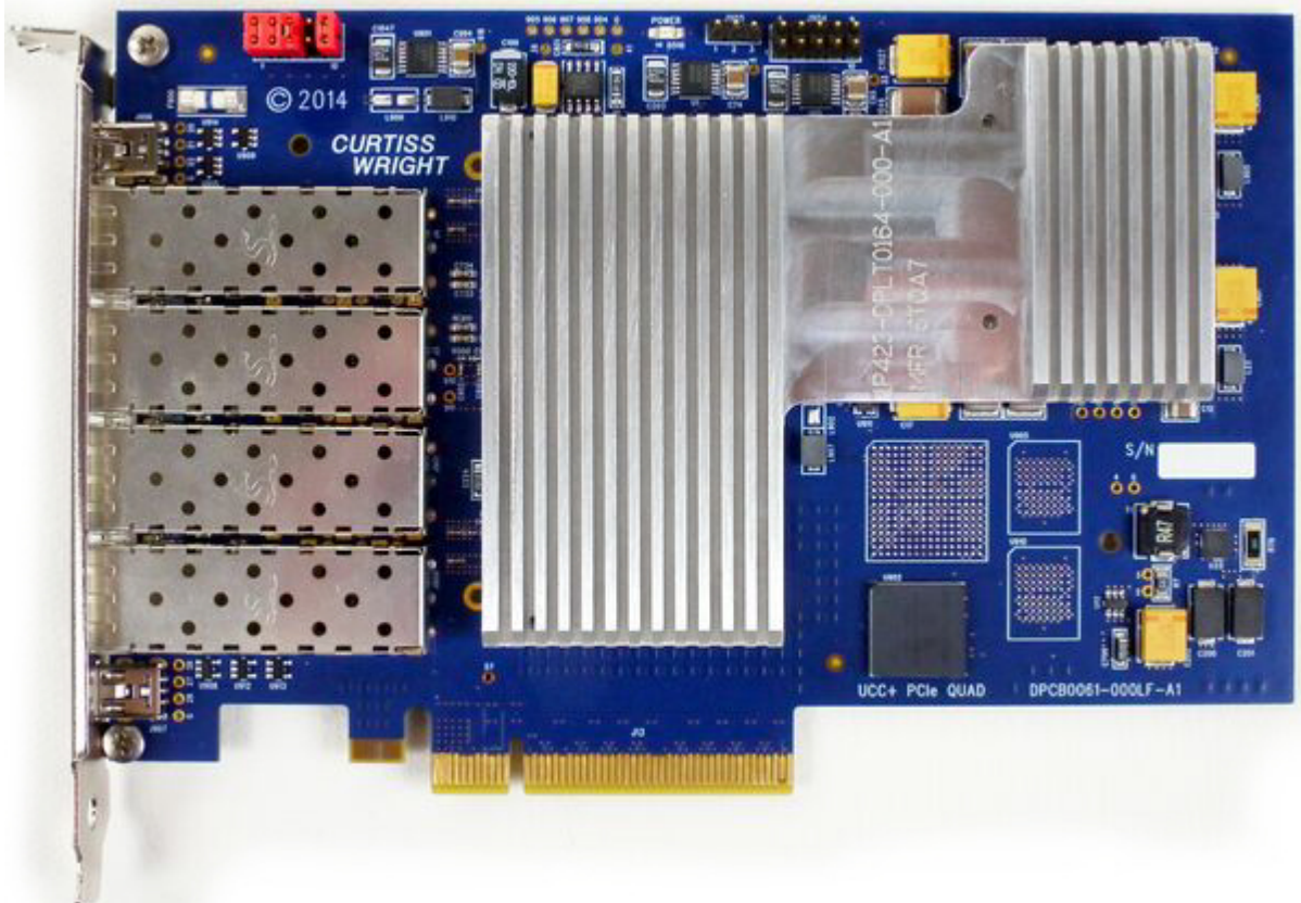
Figure 2-1 SL240 PCIe 100 MHz Card
