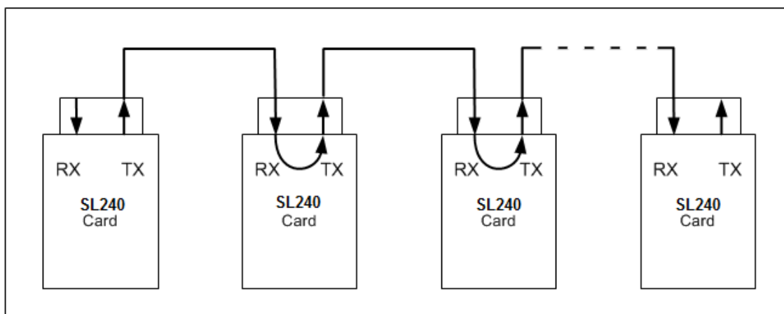
Figure 2-5 Chained Topology
