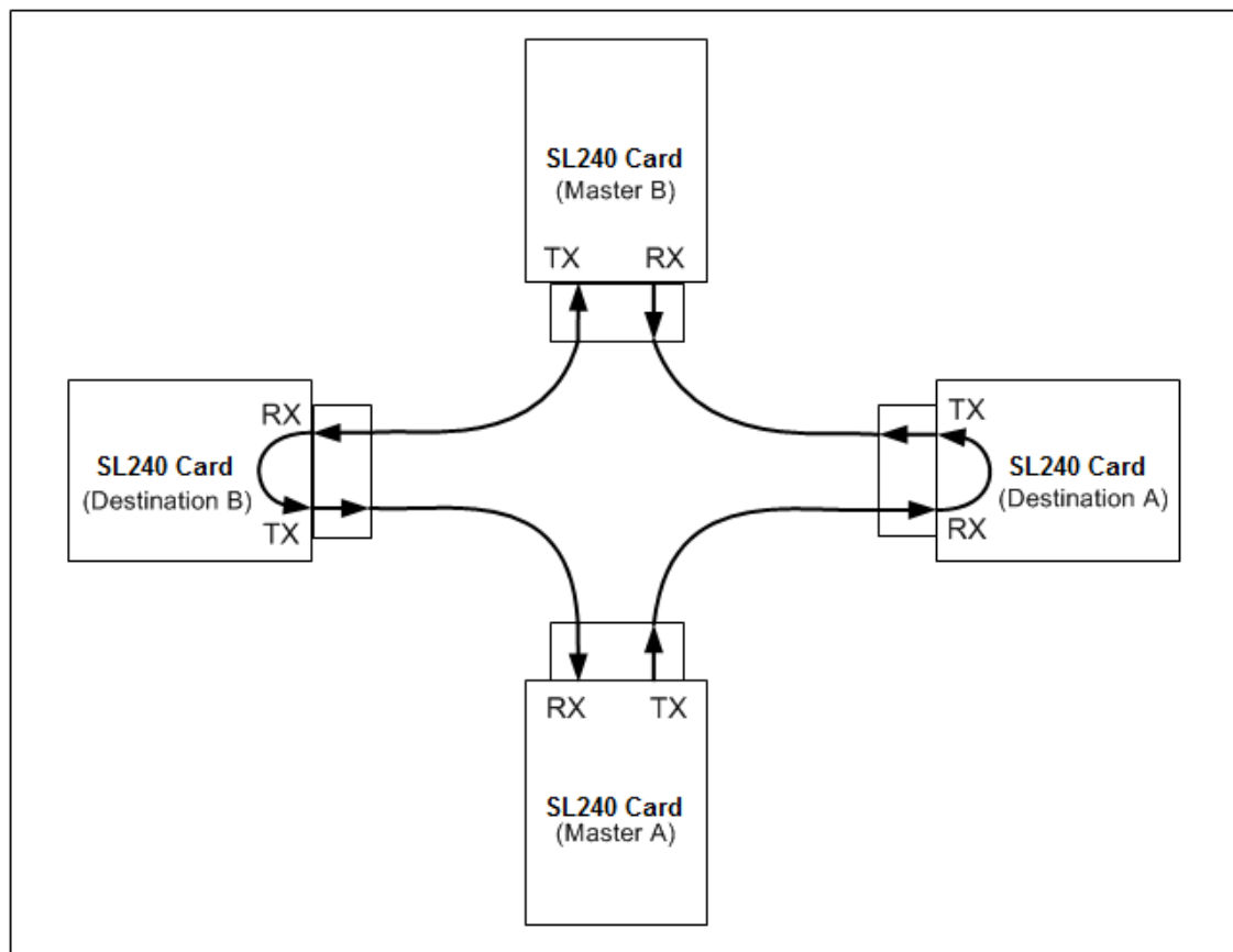
Figure 2-7 Multiple Master Ring
