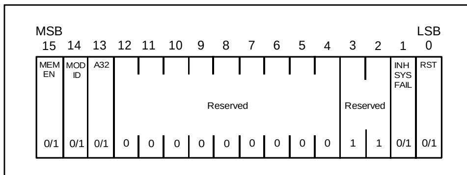
Figure 7-4 Status/Control Register
