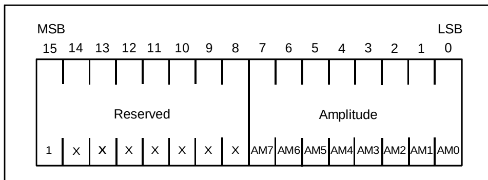
Figure 7-19 Amplitude Register
