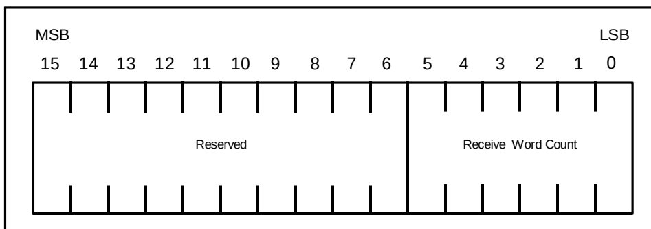
Figure 4-7 Header Word 2
