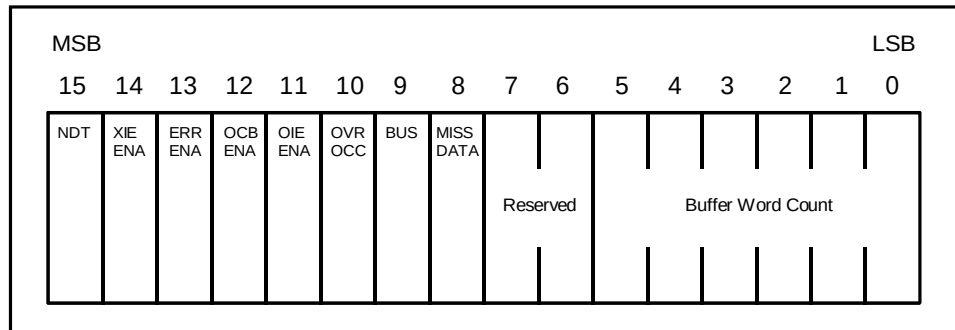
Figure 3-16 Header Word 1
