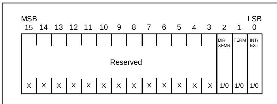
Figure 7-20 Relay Register
