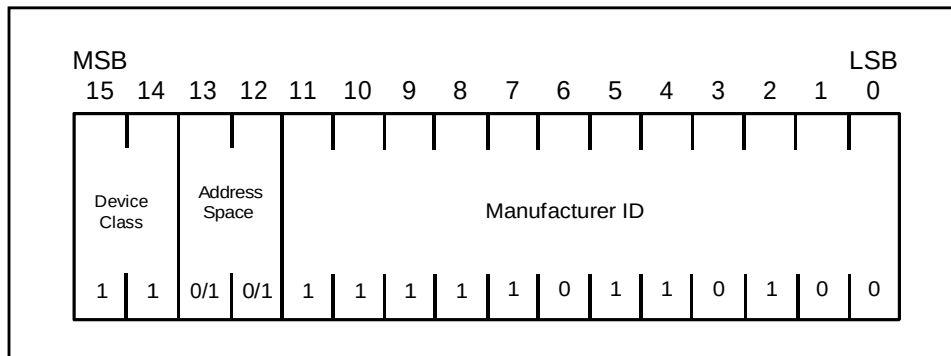
Figure 7-2 ID Register
