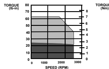
DSM030/YSM323 @ 115VAC**
