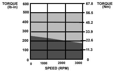
DSM1150/FSM630 @ 230 VAC
