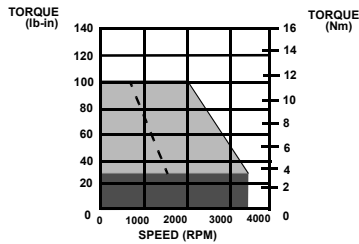
DSM030/FSM460 @ 230 VAC
