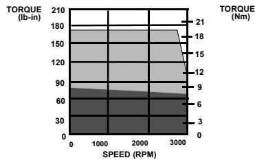
DSM175/FSM610 @ 230 VAC
