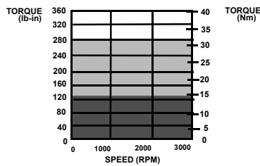
DSM175/FSM620 @ 230 VAC
