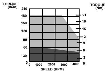
DSM175/HSM490 @ 230VAC
