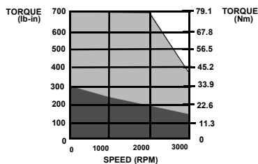
DSM1150/HSM835 @ 230VAC
