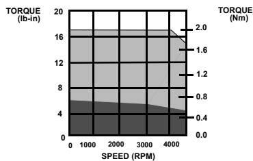
DSM030/YSM212 @ 115VAC
