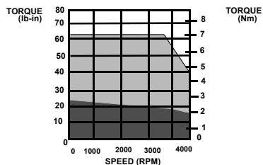
DSM030/YSM323 @ 230VAC
