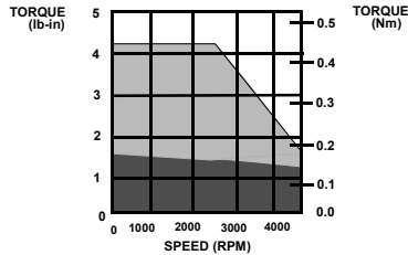
DSM015/YSM103 @ 115VAC
