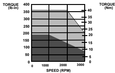
DSM1150/HSM620 @ 230VAC
