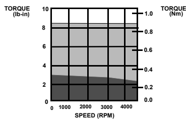
DSM030/YSM206 @ 115VAC
