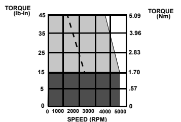
DSM015/NSM4214 @ 230VAC
