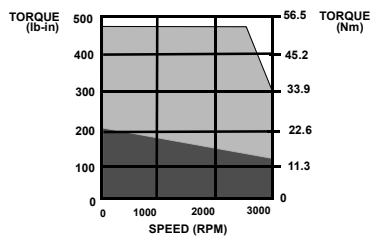
DSM1150/HSM630 @ 230VAC
