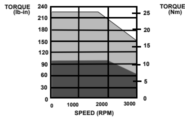
DSM175/HSM620 @ 230VAC
