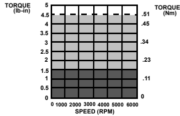
DSM007/NSM2304 @ 115VAC
