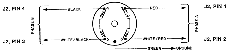
4-Lead Motors
