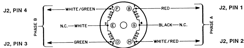
6-Lead Motors
