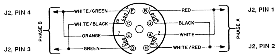
8-Lead Motors, Parallel Connections
