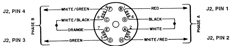
8-Lead Motors, Series Connections
