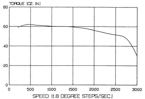
MICROSTEP WITH A 3 AMP SETTING
