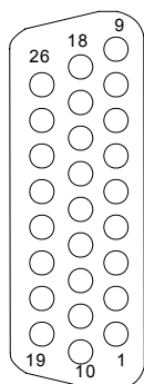
(J4 Connector view from front of drive.)
