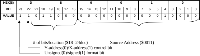
MACRO MI11x Parallel Word Example: Signed 24-bit Absolute MLDT $0010
