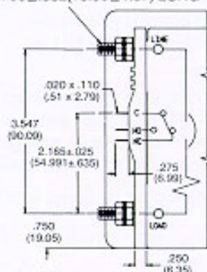
AUXILIARY SWITCH
