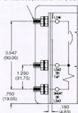
SHUNT TAP
