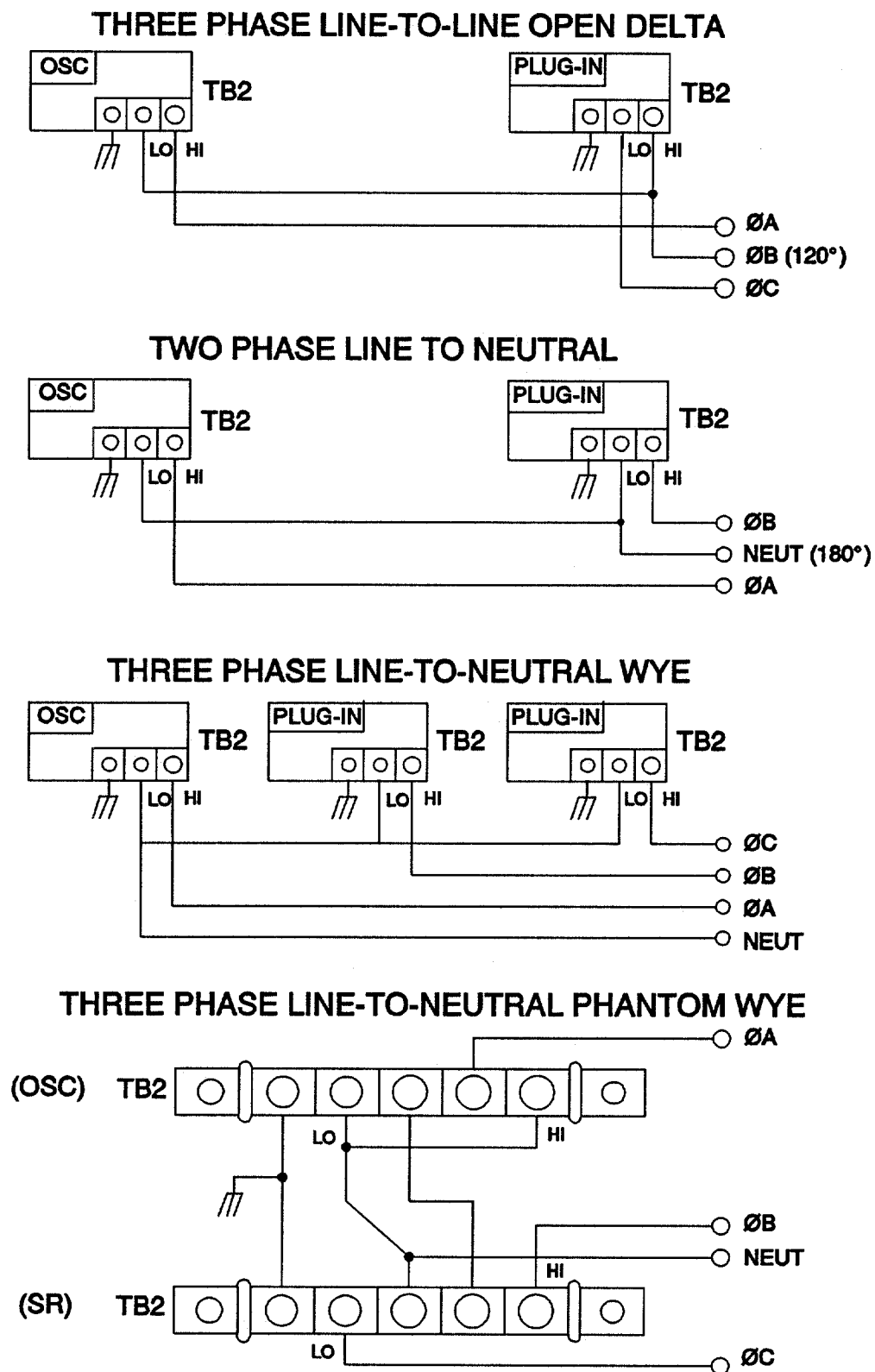
Figure 2-14. System Interconnections
