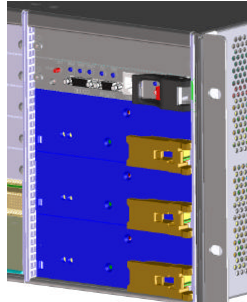
With Pluggable Shelf Manager Module (4HP) and Filler Panel (4HP)
