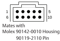
Figure 4. Connector J1
