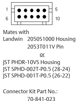
Figure 3. Connector J2
