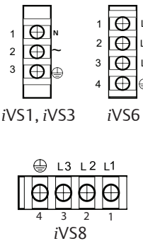
Figure 1. AC Input
