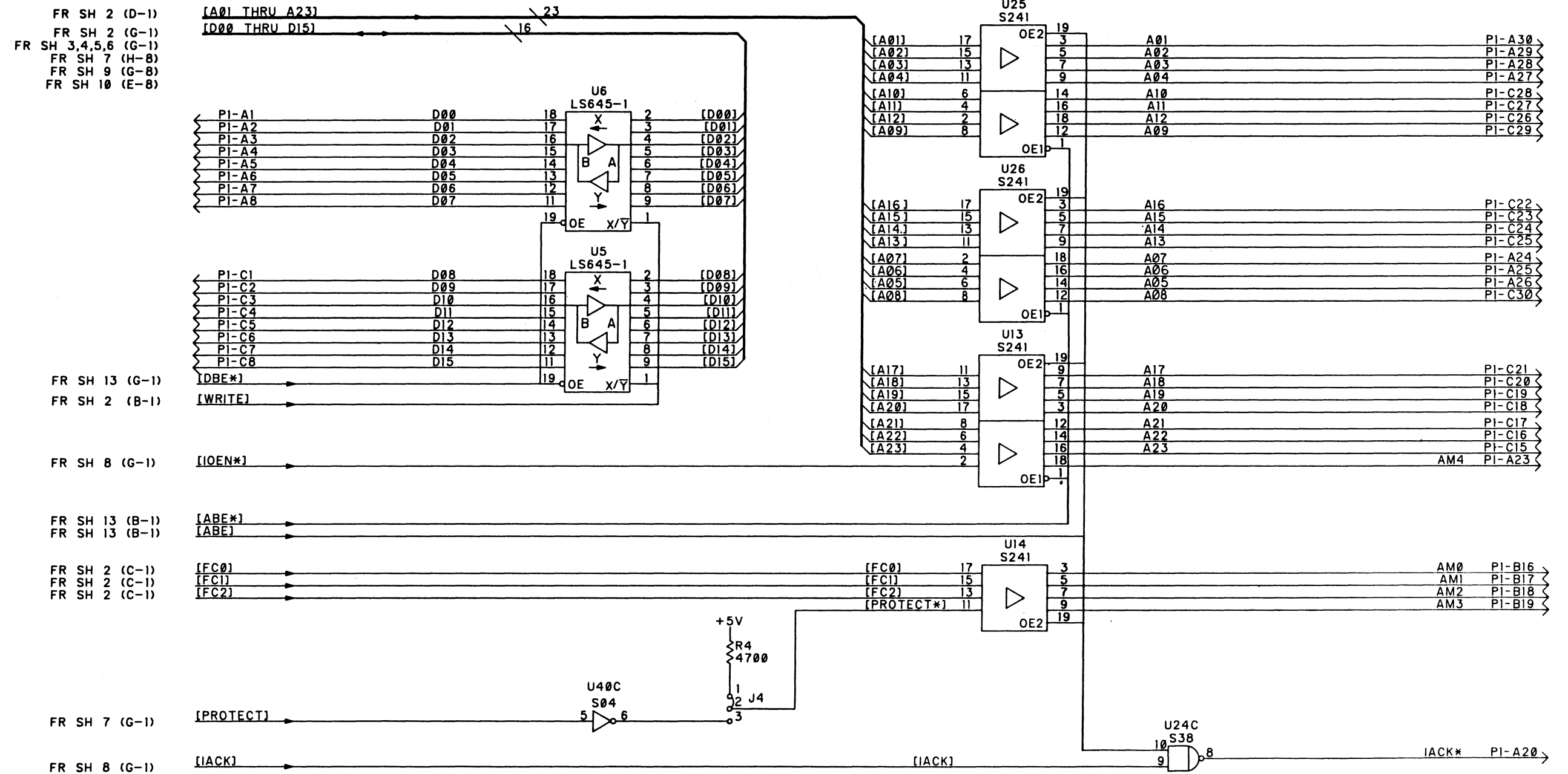
VME INTERFACE 63EW3047B REV A SH 14 OF 14
