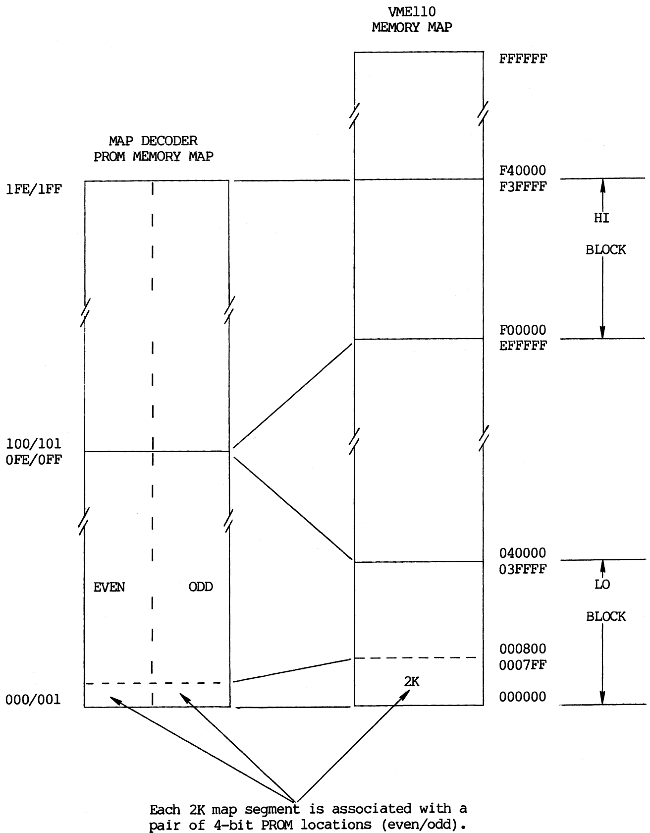
FIGURE 2-31. Relationship of Map Decoder PROM Addresses to VME110 Memory Map
