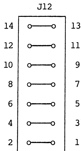
FIGURE 2-12. VMEbus Interrupt Enable Header (J12)
