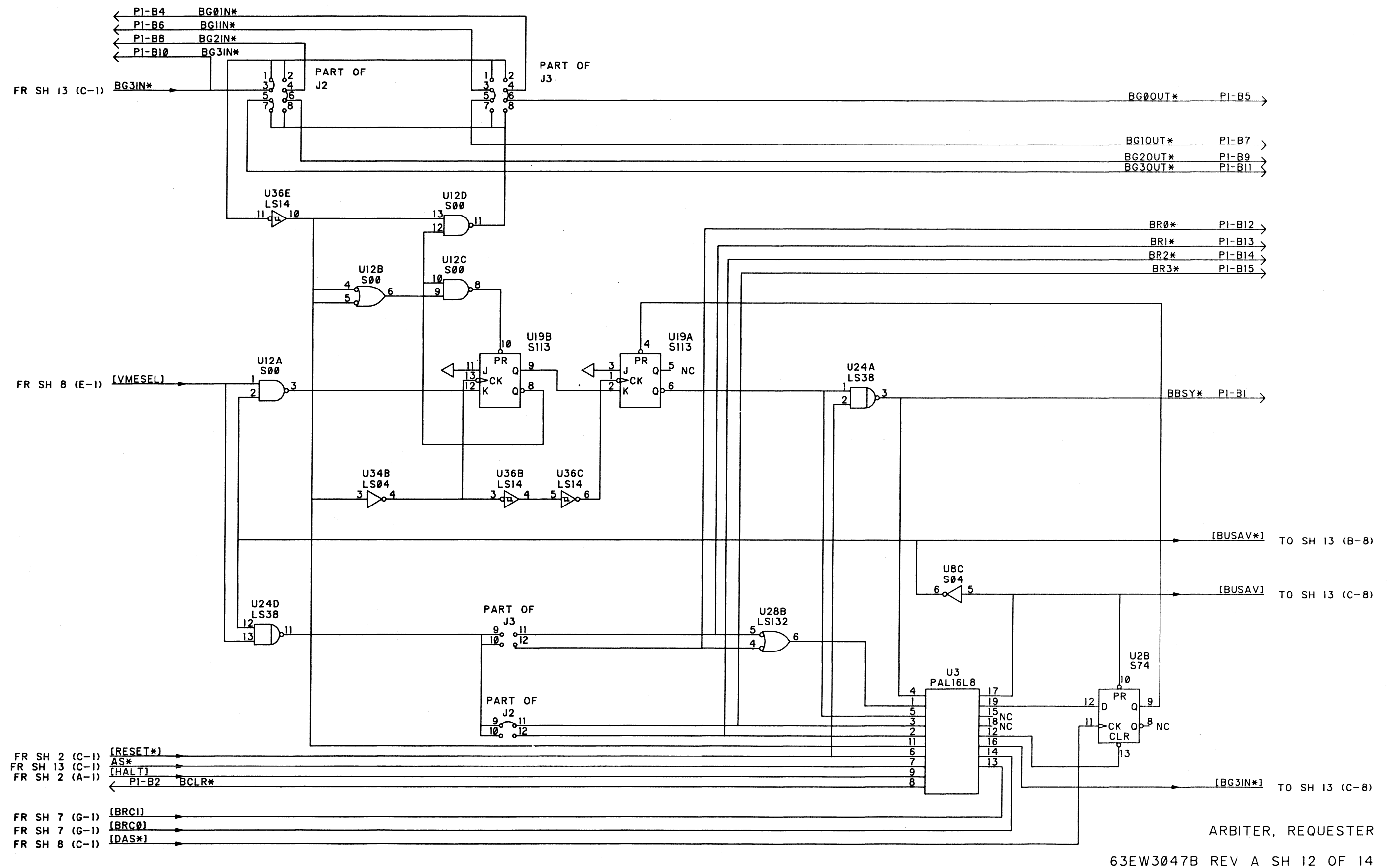
FIGURE 5-2. VME110 Module Schematic Diagram (Sheet 12 of 14) 5-37/5-38
