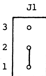
FIGURE 2-2. MPU Clock Speed Header (J1)
