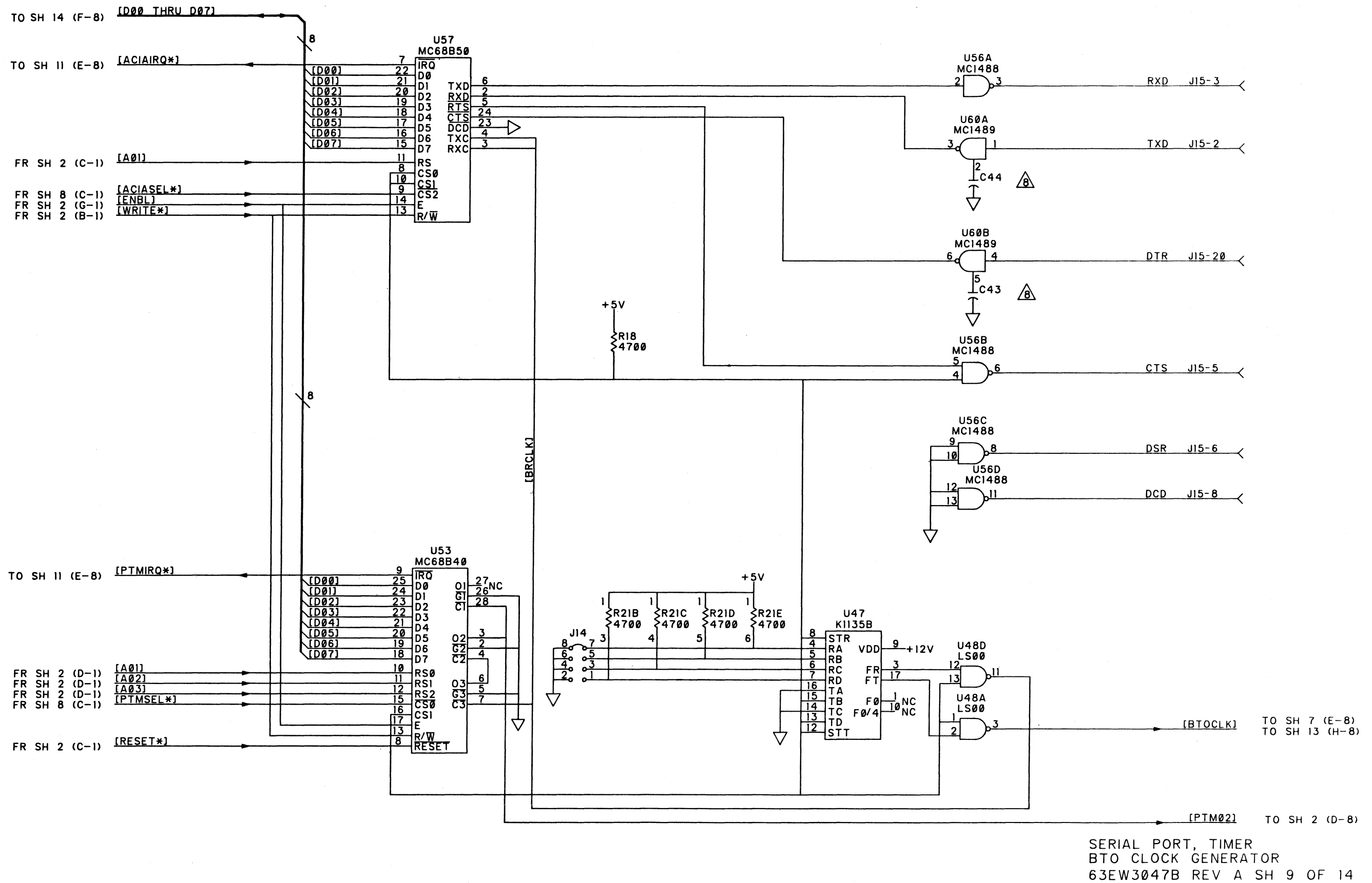
FIGURE 5-2. VME110 Module Schematic Diagram (Sheet 9 of 14) 5-31/5-32
