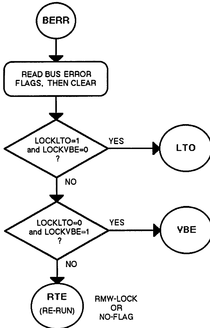
FIGURE 1. Bus Error Exception Handler Flowchart for MVME133XT
