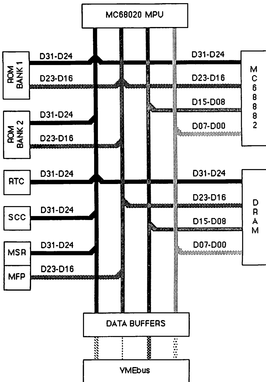
FIGURE 4-2. MVME133XT Data Bus Structure
