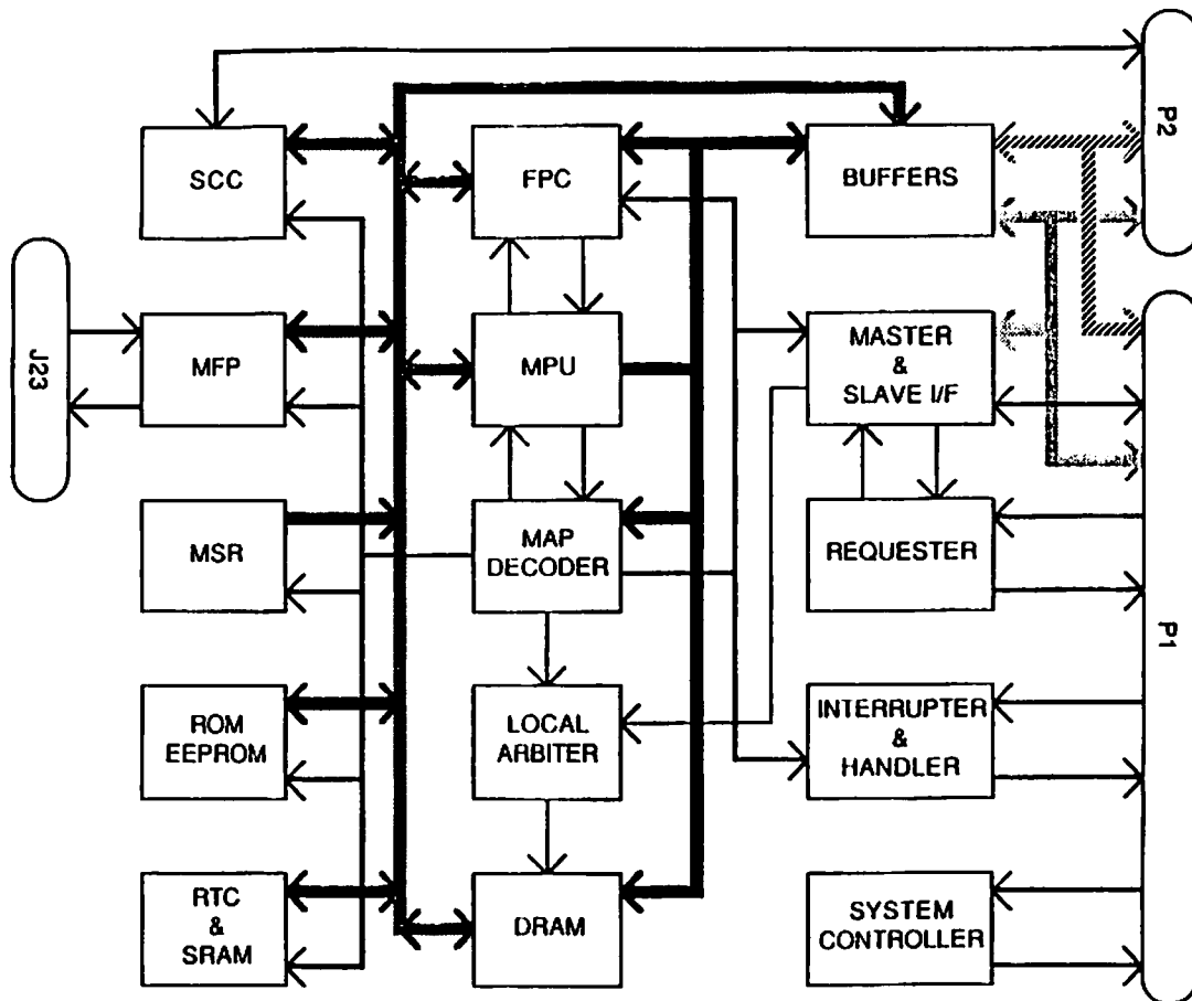
FIGURE 4-1. MVME133XT Block Diagram
