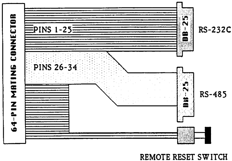
FIGURE 2-2. Cabling Connections to P2, Suggestion 1
