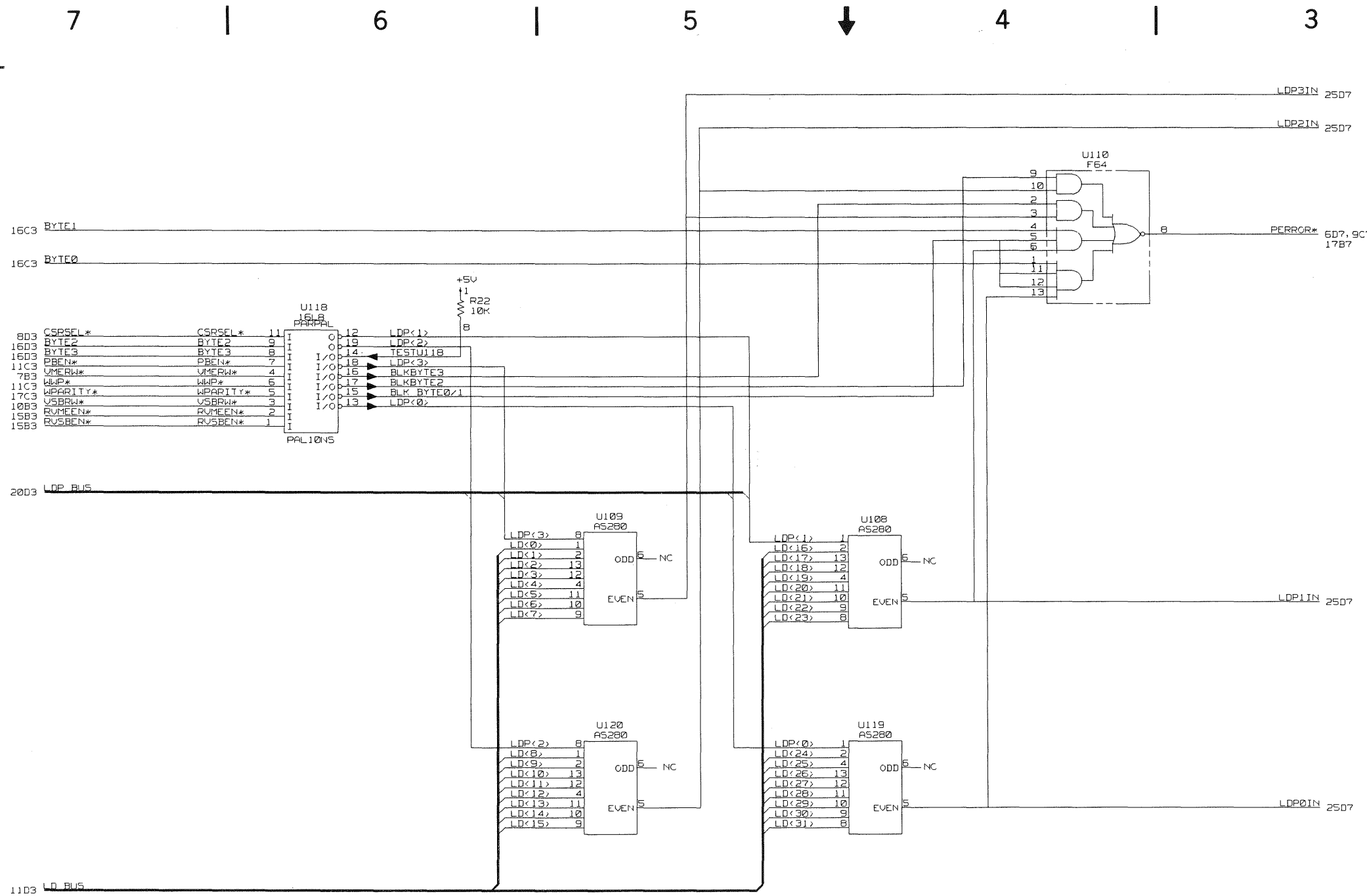
PARITY GENERATION 63DW3588B0C REV A SH 19 OF 25 FIGURE 4-2. MVME224A SCHEMATIC DIAGRAM (SHEET 19 OF 25)
