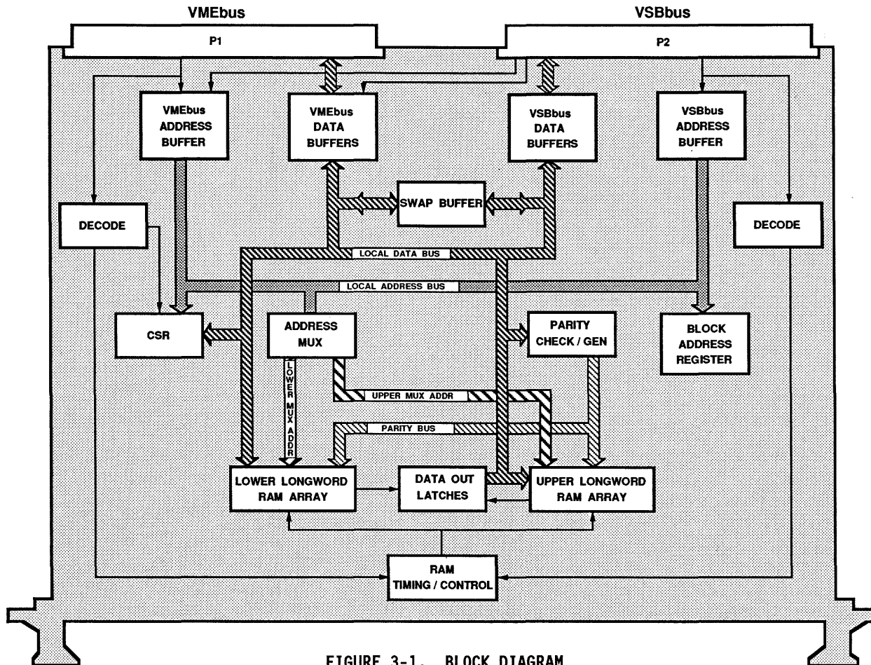
FIGURE 3-1. BLOCK DIAGRAM
