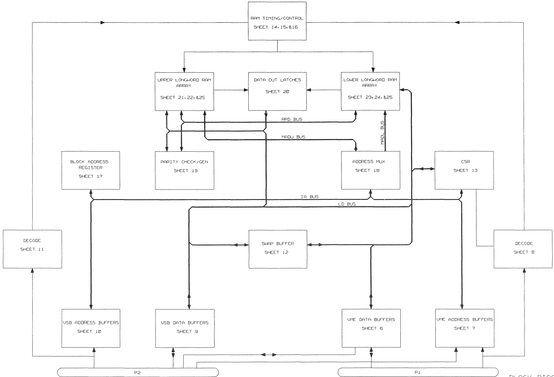
FIGURE 4-2. MVME224A SCHEMATIC DIAGRAM (SHEET 5 OF 25)
