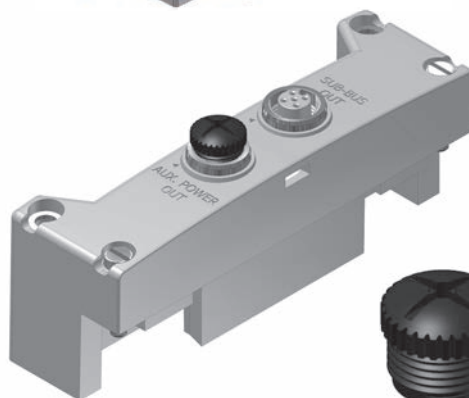
Dust Cover - M12 Male 230-647
