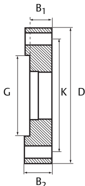
Recessed face
