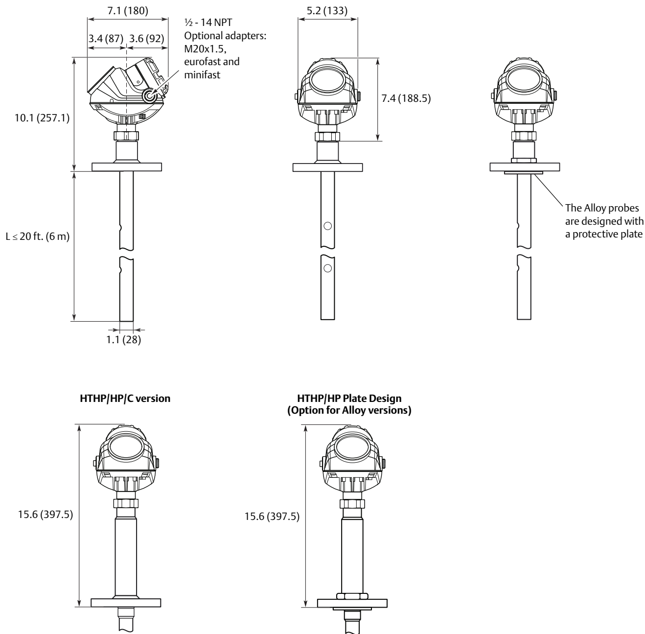
Figure 14. Coaxial Probe with Flange Connection
