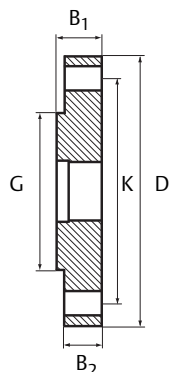
Raised face
