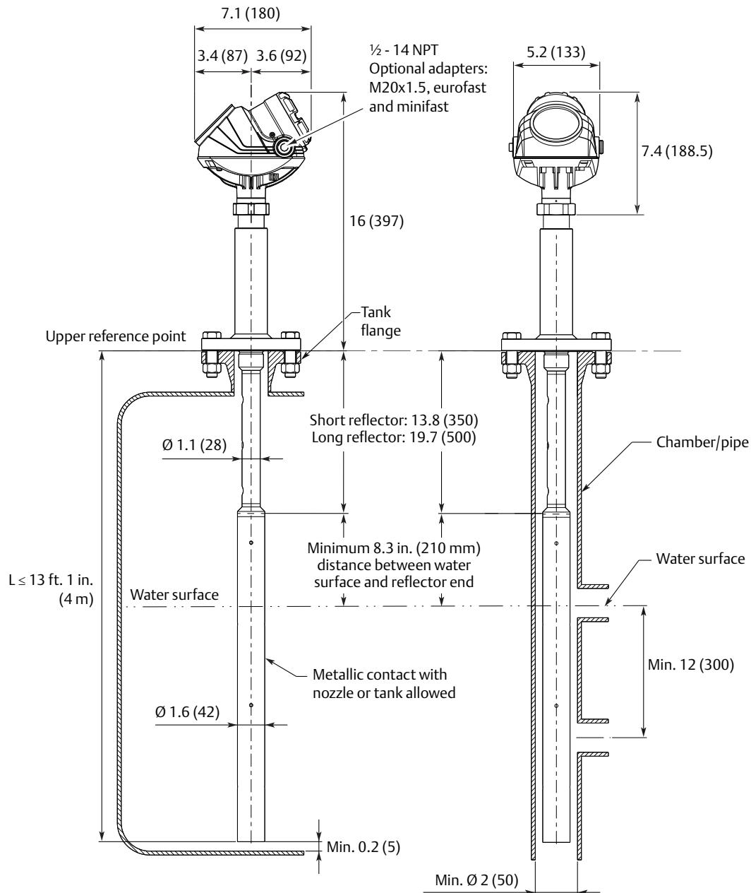
Figure 16. Integrated Still Pipe Vapor Probe for 3-in. Chambers and above
