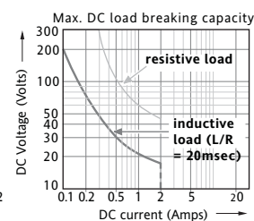
Graph 2 DC ratings
