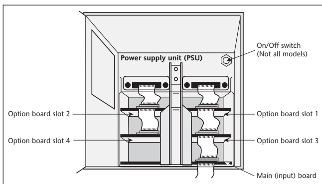
Exploded view
