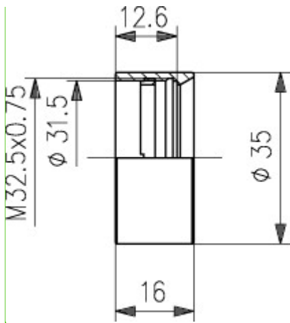
Technical drawing of part number G063668000
