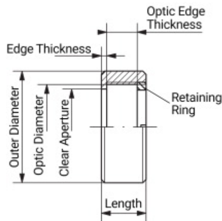
General technical drawing of the different mounts
