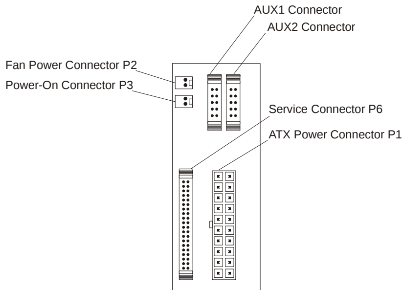
Figure 29: Location of Non-CPCI Connectors on Front Side of H.110 Backplane
